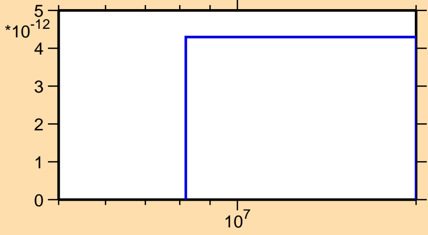
\sigma vs. E for ^{114}\text{Te}(\text{mt } 34)
