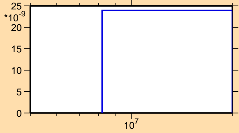
\sigma vs. E for ^{114}\text{Te}(\text{mt } 45)
