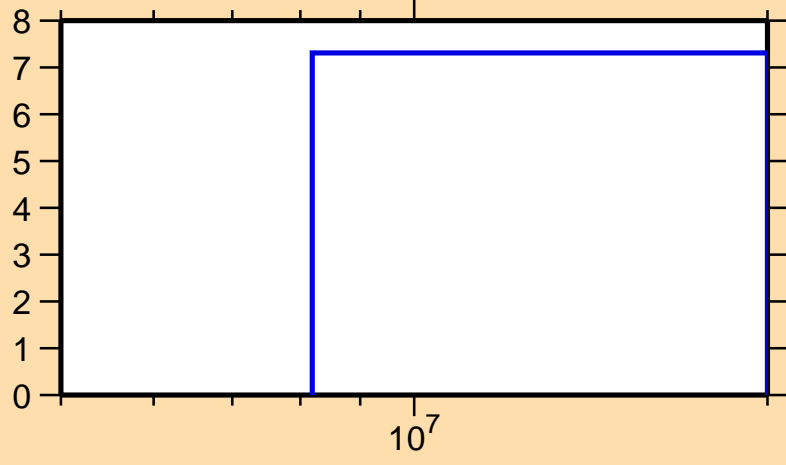
\Delta\sigma/\sigma vs. E for ^{114}\text{Te}(n,\text{tot.})
