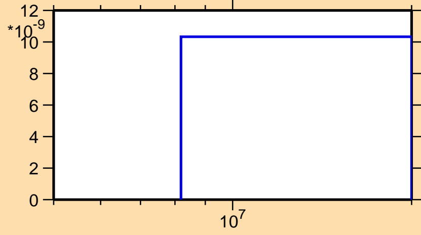
\sigma vs. E for ^{114}\text{Te}(n,nd)
