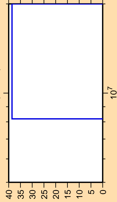
\Delta\sigma/\sigma vs. E for ^{114}\text{Te}(\text{mt } 34)
