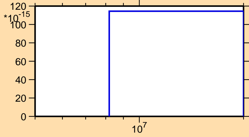
\sigma vs. E for ^{114}\text{Te}(n,nt)
