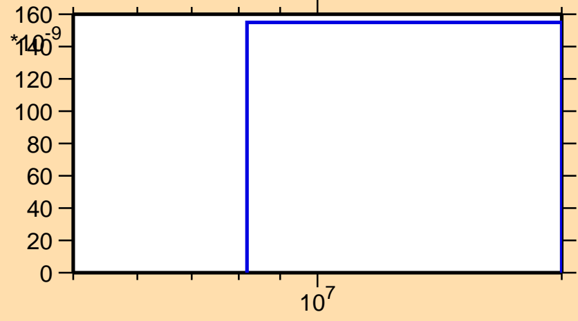
\sigma vs. E for ^{114}\text{Te}(n,2np)
