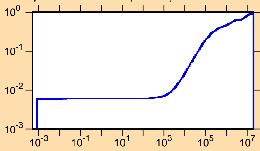
\mu vs. E for ^{116}\text{Te}(\text{mt251})
