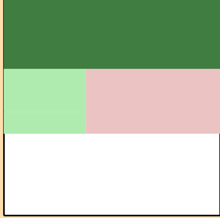
\Delta\sigma/\sigma vs. E for ^{116}\text{Te}(n,\text{nonel.})
