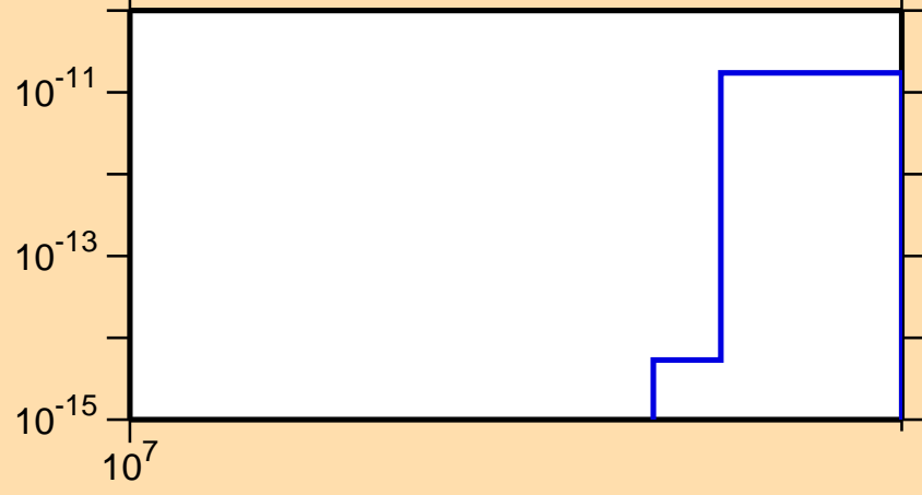
\sigma vs. E for ^{116}\text{Te} (mt 34)
