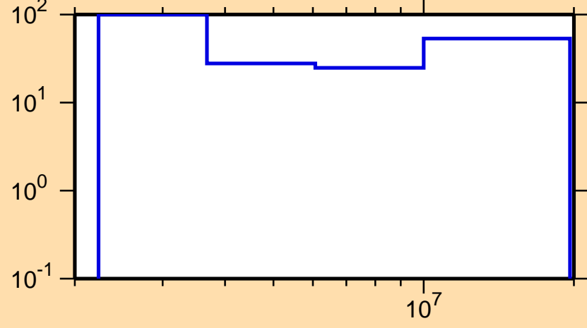
\Delta\sigma/\sigma vs. E for ^{116}\text{Te}(n,n\text{cont.})
