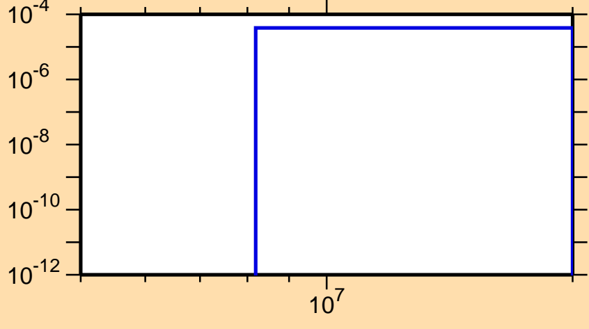
\sigma vs. E for ^{116}\text{Te}(n,t)
