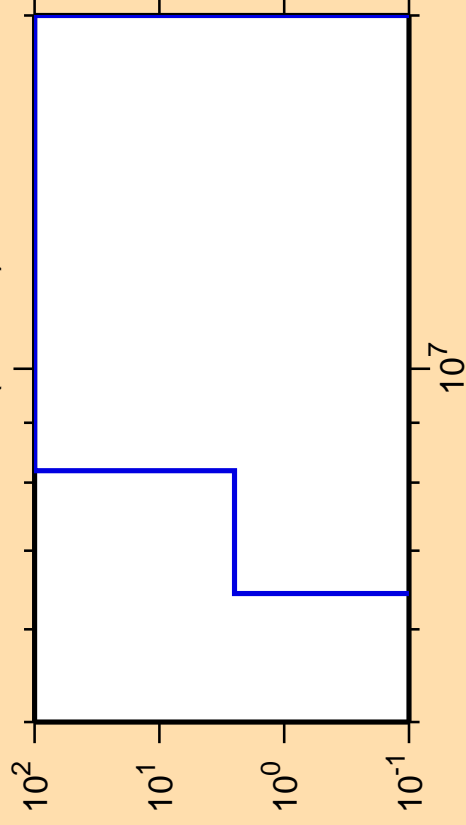
\Delta\sigma/\sigma vs. E for ^{116}\text{Te}(n,\text{He3})
