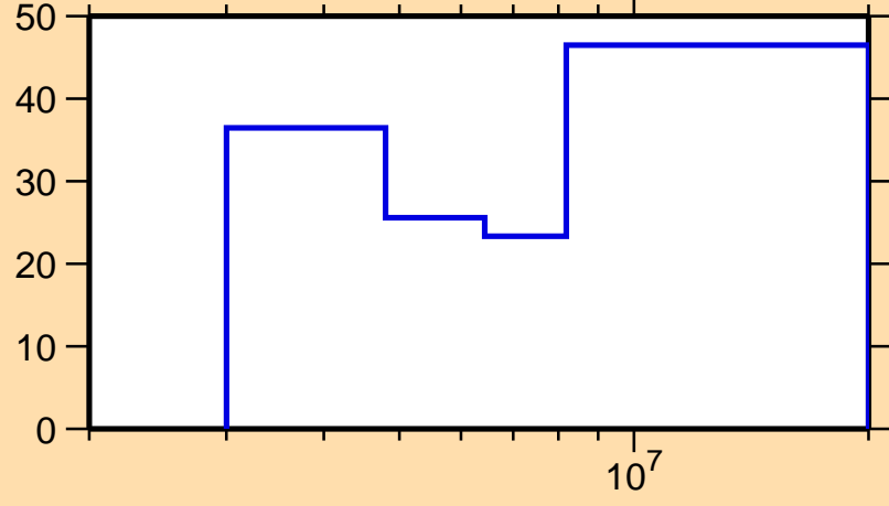
\Delta\sigma/\sigma vs. E for ^{116}\text{Te}(n,ncont.)
