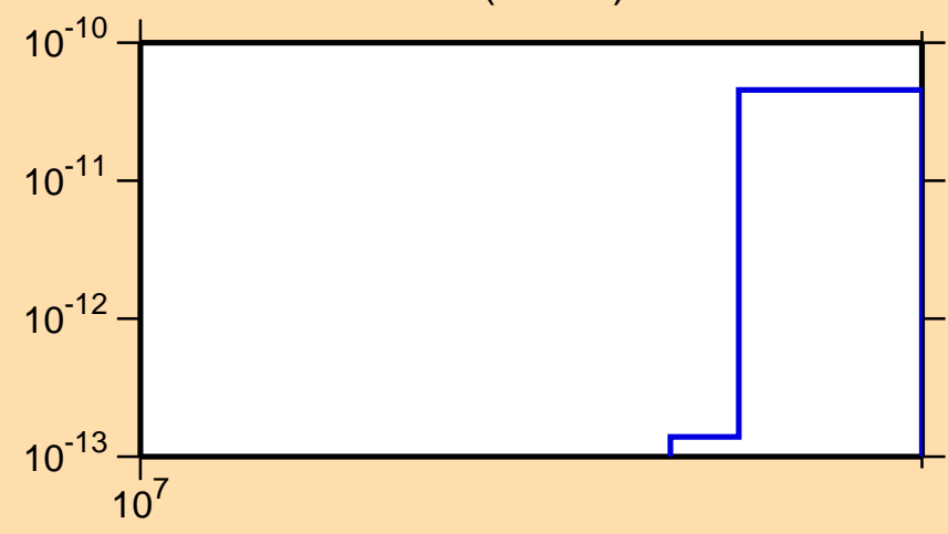
\sigma vs. E for ^{118}\text{Te} (mt 45)
