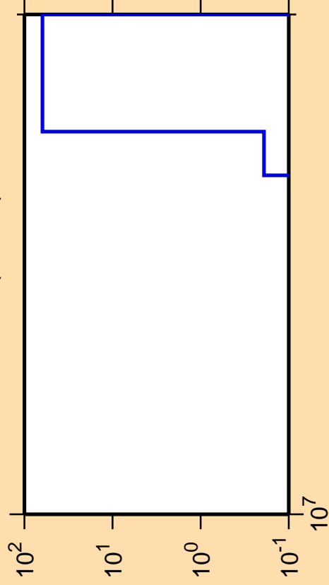
\Delta\sigma/\sigma vs. E for ^{118}\text{Te} (mt 45)
