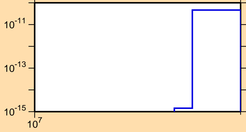
\sigma vs. E for ^{118}\text{Te}(n,\text{pt})
