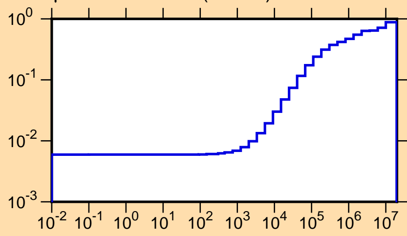
\mu vs. E for ^{118}\text{Te}(\text{mt251})
