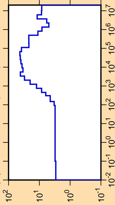
\Delta\mu/\mu vs. E for ^{118}\text{Te}(\text{mt251})
