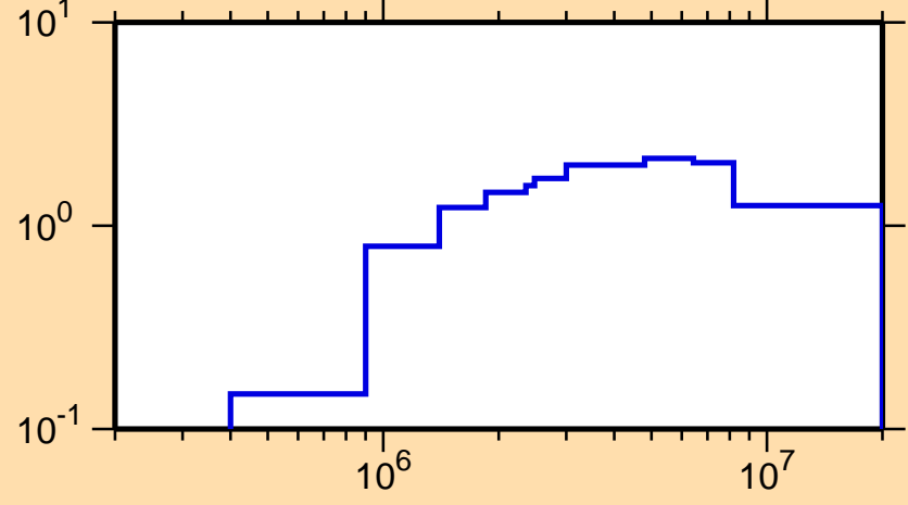
\sigma vs. E for ^{118}\text{Te}(n,\text{inel.})
