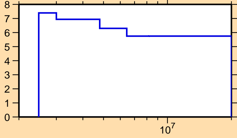
\Delta\sigma/\sigma vs. E for ^{118}\text{Te}(n,\text{nonel.})
