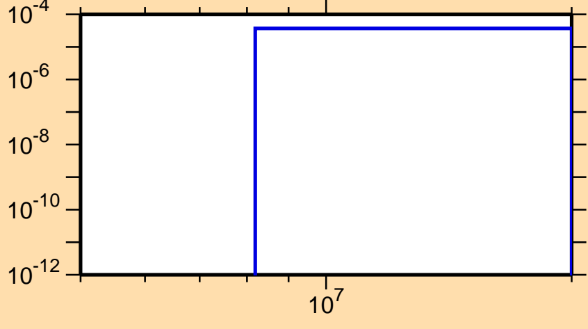
\sigma vs. E for ^{118}\text{Te}(n,t)
