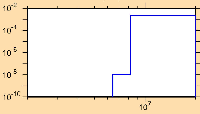
\sigma vs. E for ^{118}\text{Te}(n,d)
