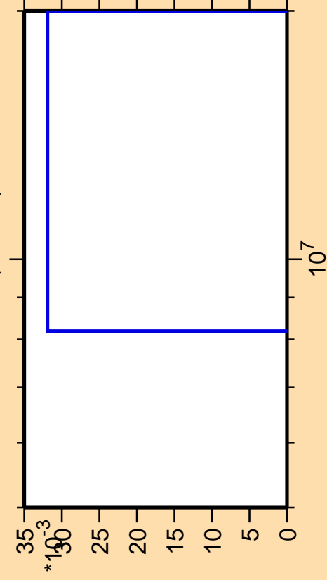
\Delta\sigma/\sigma vs. E for ^{118}\text{Te}(\text{mt } 34)
