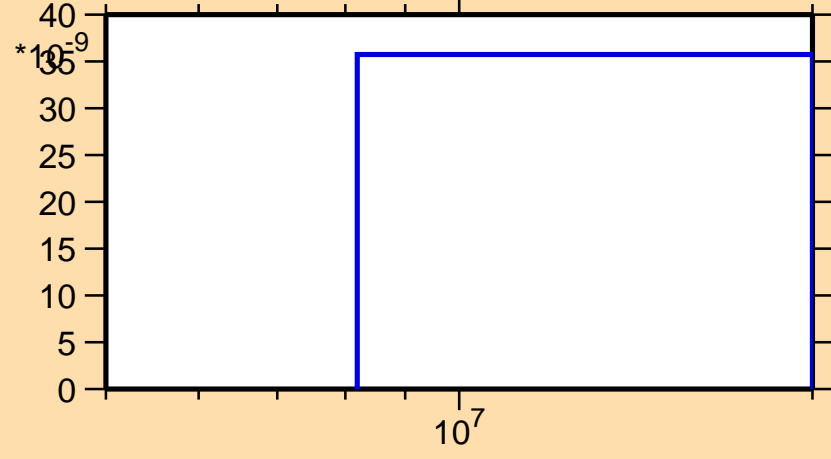
\sigma vs. E for ^{118}\text{Te}(n,2n\alpha)
