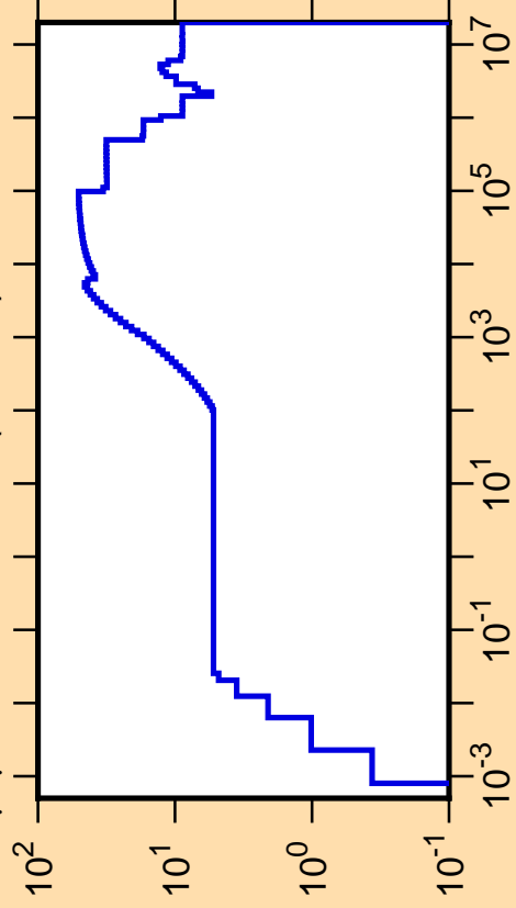
\Delta\mu/\mu vs. E for ^{119}\text{Te}(\text{mt251})
