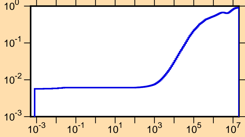
\mu vs. E for ^{119}\text{Te}(\text{mt251})
