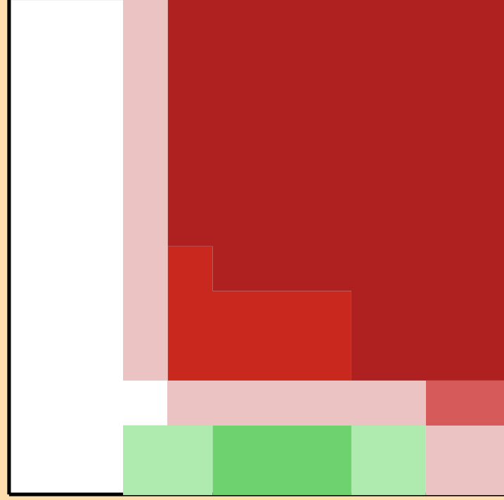
\Delta\sigma/\sigma vs. E for ^{119}\text{Te}(n,2n)
