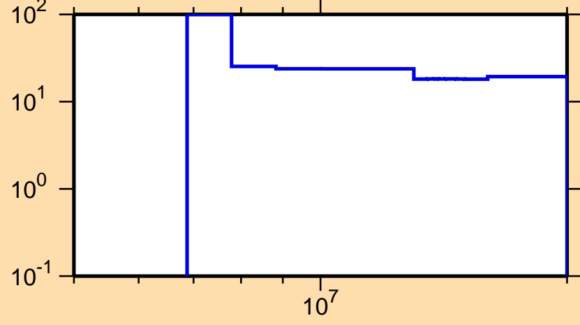
\Delta\sigma/\sigma vs. E for ^{119}\text{Te}(n,2n)
