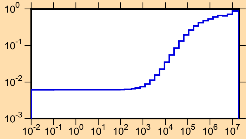
\mu vs. E for ^{119}\text{Te}(\text{mt251})
