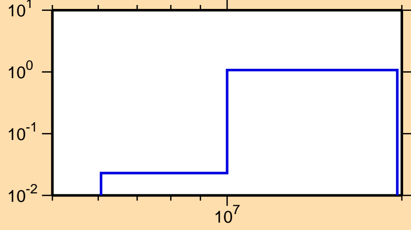
\sigma vs. E for ^{119}\text{Te}(n,2n)
