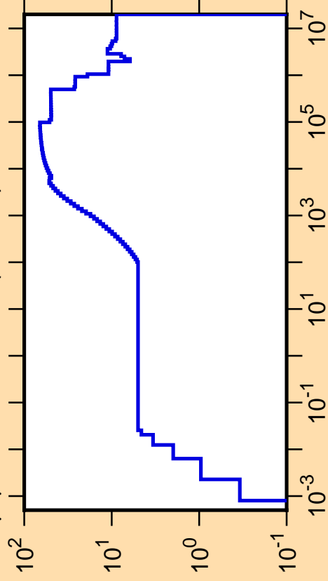
\Delta\mu/\mu vs. E for ^{121}\text{Te}(\text{mt251})
