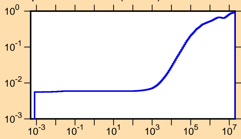
\mu vs. E for ^{121}\text{Te}(\text{mt251})
