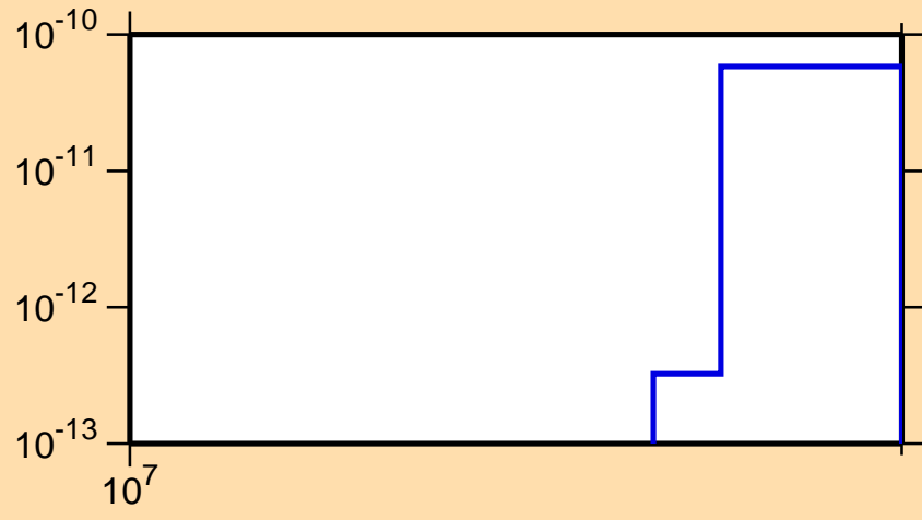
\sigma vs. E for ^{121}\text{Te}(n,\text{pd})
