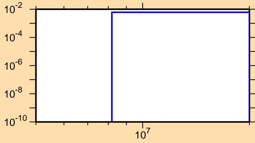
\sigma vs. E for ^{121}\text{Te}(n,np)
