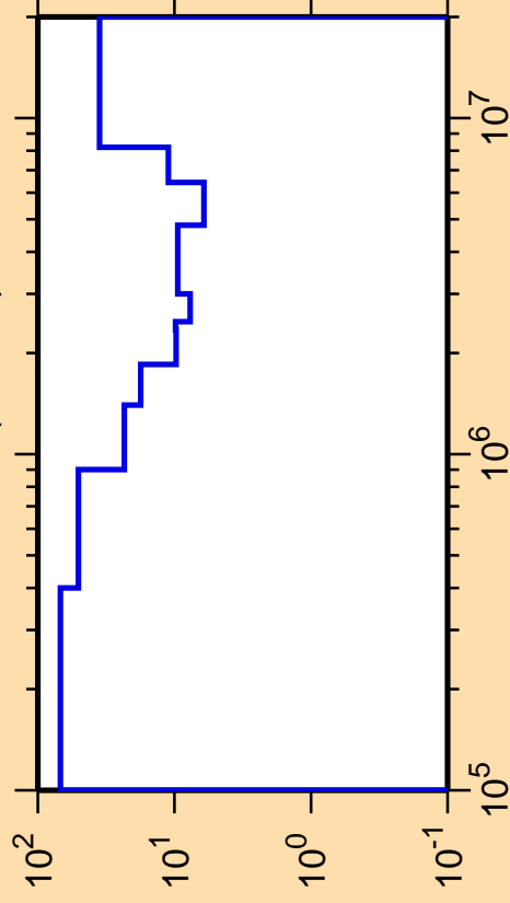
\Delta\sigma/\sigma vs. E for ^{121}\text{Te}(n,\text{inel.})
