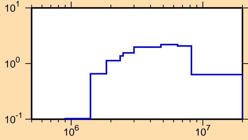
\sigma vs. E for ^{121}\text{Te}(n,n\text{cont.})
