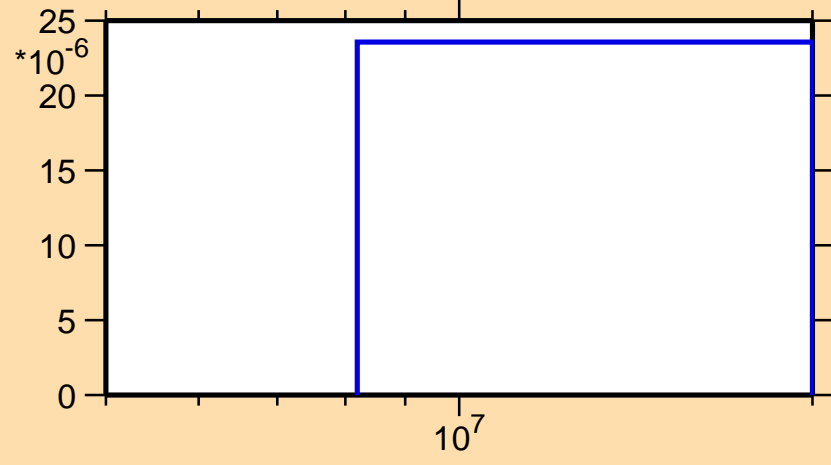
\sigma vs. E for ^{121}\text{Te}(n,3n)
