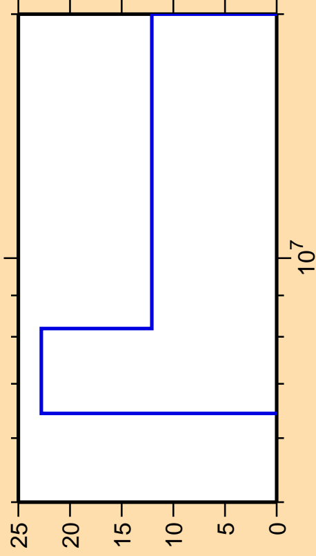
\Delta\sigma/\sigma vs. E for ^{121}\text{Te}(n,2n)
