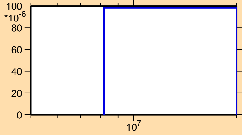
\sigma vs. E for ^{121}\text{Te}(n,t)
