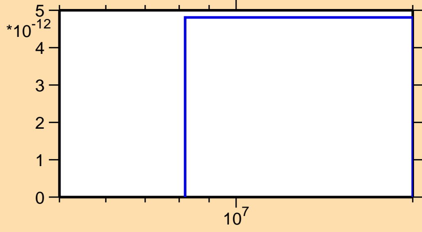
\sigma vs. E for ^{121}\text{Te}(n,nt)
