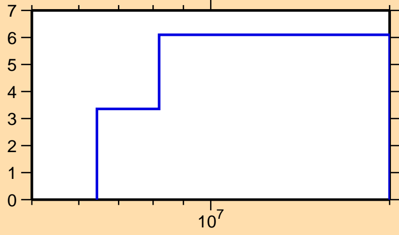
\Delta\sigma/\sigma vs. E for ^{121}\text{Te}(n,\text{tot.})
