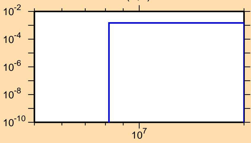
\sigma vs. E for ^{121}\text{Te}(n,d)
