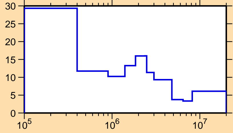
\Delta\sigma/\sigma vs. E for ^{121}\text{Te}(n,\text{tot.})
