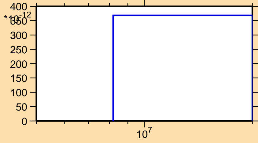
\sigma vs. E for ^{121}\text{Te}(n,p\alpha)
