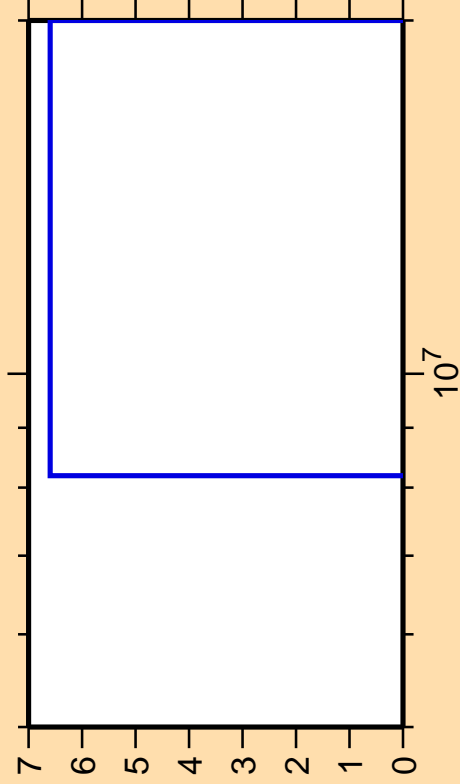
\Delta\sigma/\sigma vs. E for ^{121}\text{Te}(n,\text{pt})
