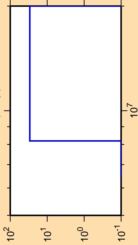
\Delta\sigma/\sigma vs. E for ^{121}\text{Te}(n,np)
