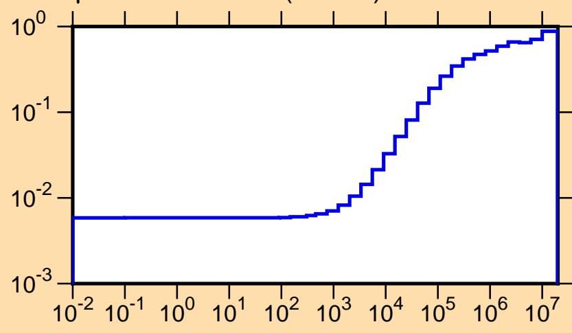
\mu vs. E for ^{123}\text{Te}(\text{mt251})
