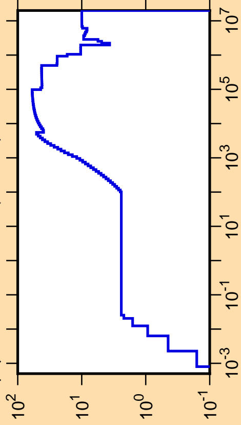
\Delta\mu/\mu vs. E for ^{129}\text{Te}(\text{mt251})
