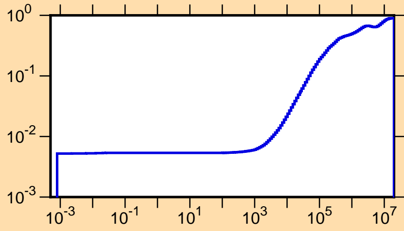
\mu vs. E for ^{129}\text{Te}(\text{mt251})
