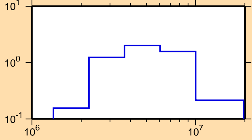
\sigma vs. E for ^{129}\text{Te}(n,n\text{cont.})
