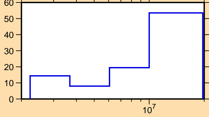
\Delta\sigma/\sigma vs. E for ^{129}\text{Te}(n,ncont.)
