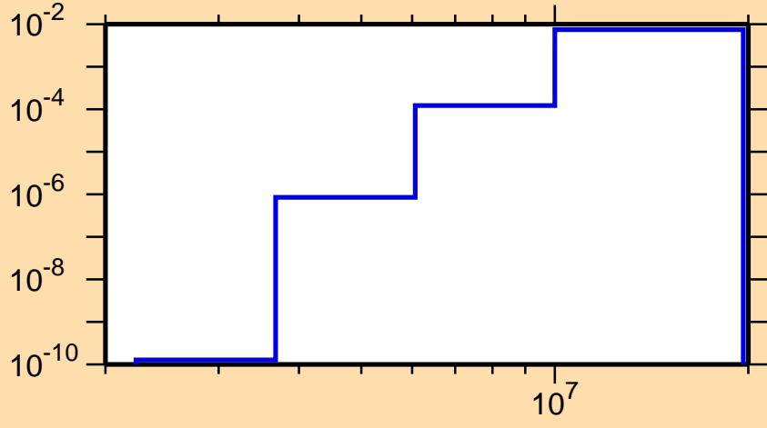
\sigma vs. E for ^{129}\text{Te}(n,p)
