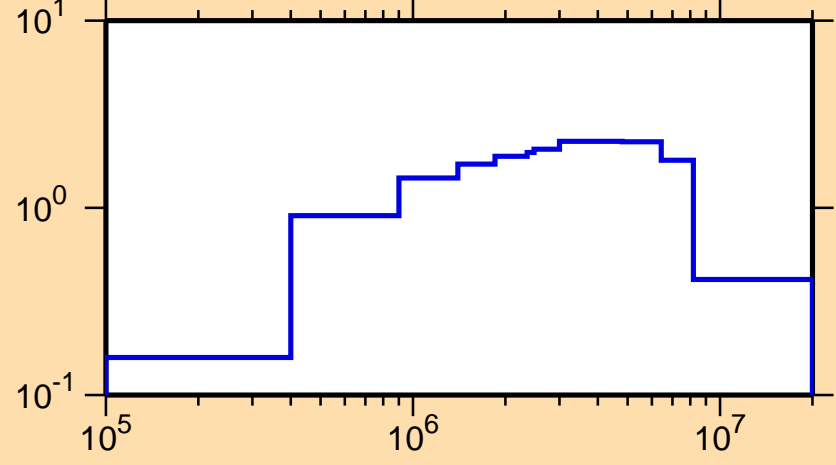
\sigma vs. E for ^{129}\text{Te}(n,\text{inel.})
