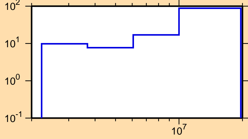
\Delta\sigma/\sigma vs. E for ^{129}\text{Te}(n,ncont.)
