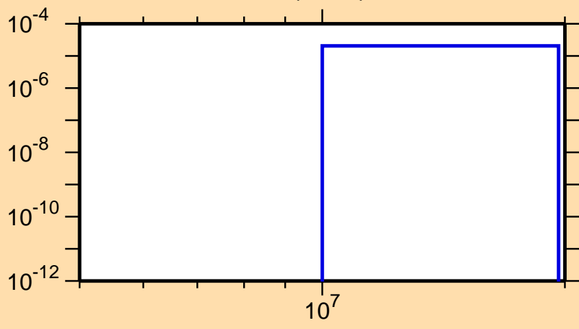
\sigma vs. E for ^{129}\text{Te}(n,\alpha)
