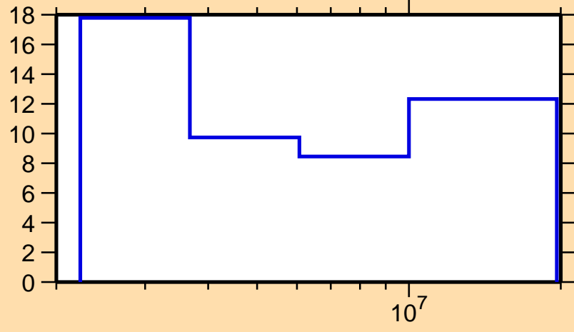
\Delta\sigma/\sigma vs. E for ^{129}\text{Te}(n,el.)
