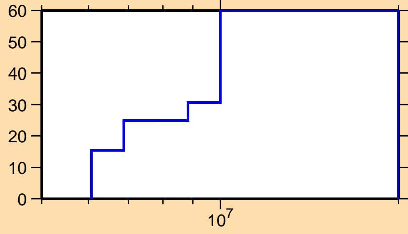
\Delta\sigma/\sigma vs. E for ^{134}\text{Te}(n,inel.)
