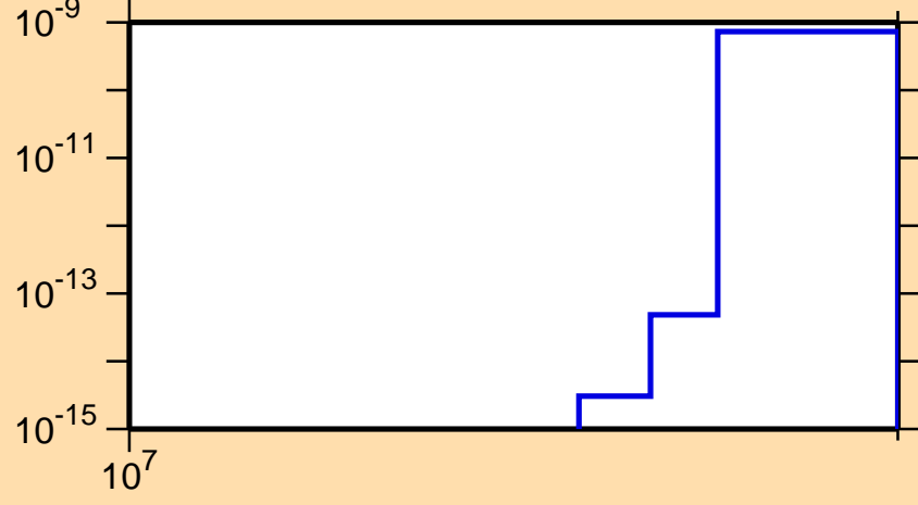
\sigma vs. E for ^{134}\text{Te}(n,nt)
