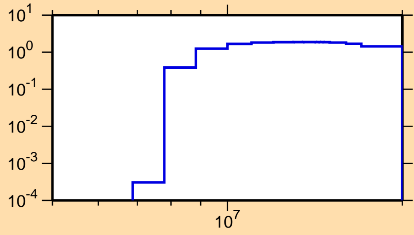
\sigma vs. E for ^{134}\text{Te}(n,2n)
