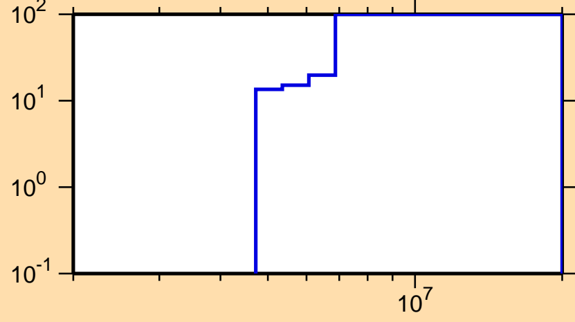
\Delta\sigma/\sigma vs. E for ^{134}\text{Te}(n,n_1)
