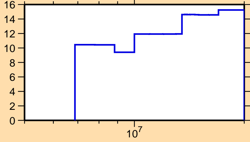
\Delta\sigma/\sigma vs. E for ^{134}\text{Te}(n,\text{tot.})
