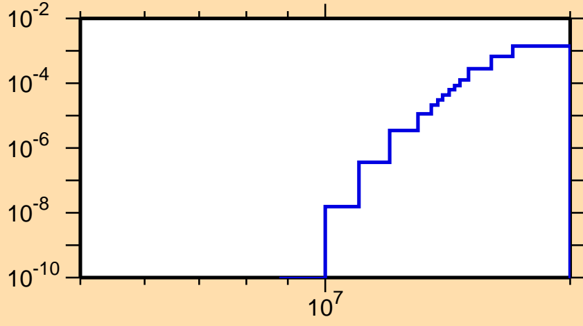
\sigma vs. E for ^{134}\text{Te}(n,p)
