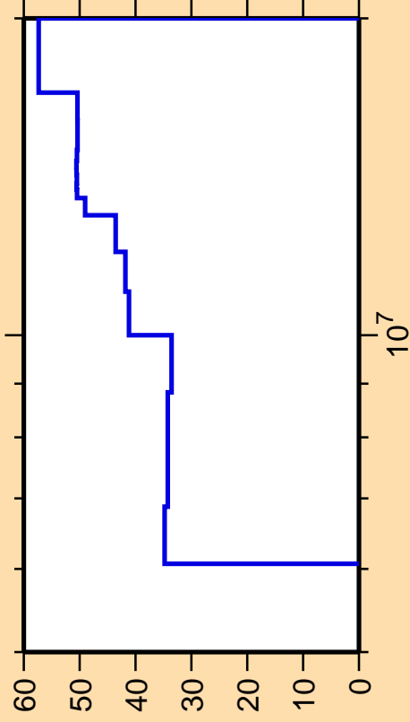
\Delta\sigma/\sigma vs. E for ^{134}\text{Te}(n,ncont.)
