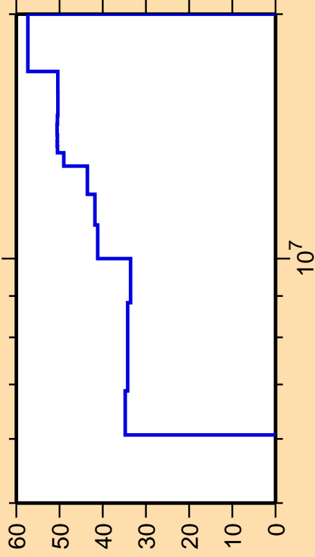
\Delta\sigma/\sigma vs. E for ^{134}\text{Te}(n,n\text{cont.})
