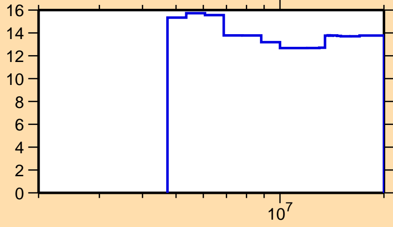
\Delta\sigma/\sigma vs. E for ^{134}\text{Te}(n,\text{nonel.})
