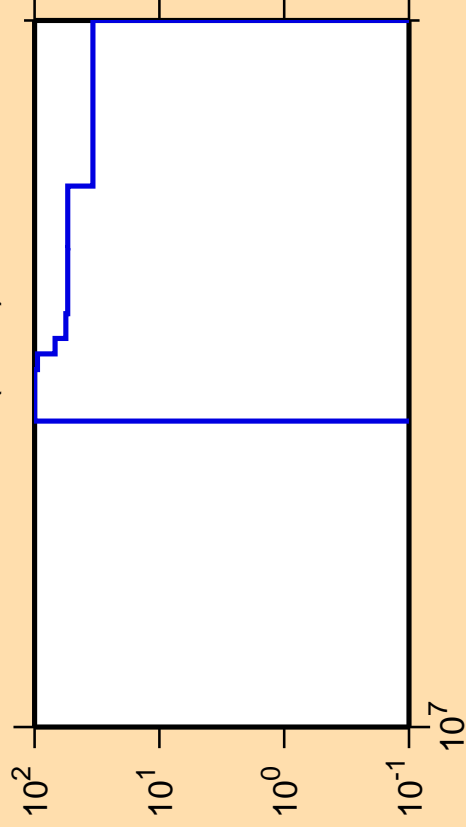
\Delta\sigma/\sigma vs. E for ^{134}\text{Te}(n,3n)
