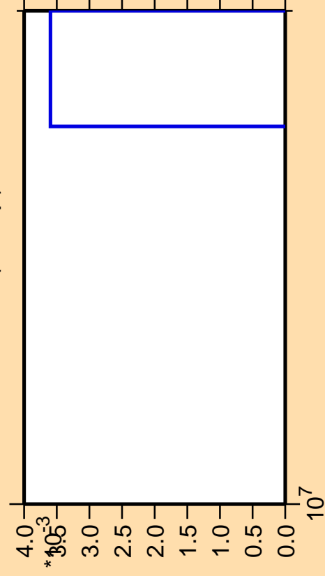
\Delta\sigma/\sigma vs. E for ^{134}\text{Te}(n,2np)
