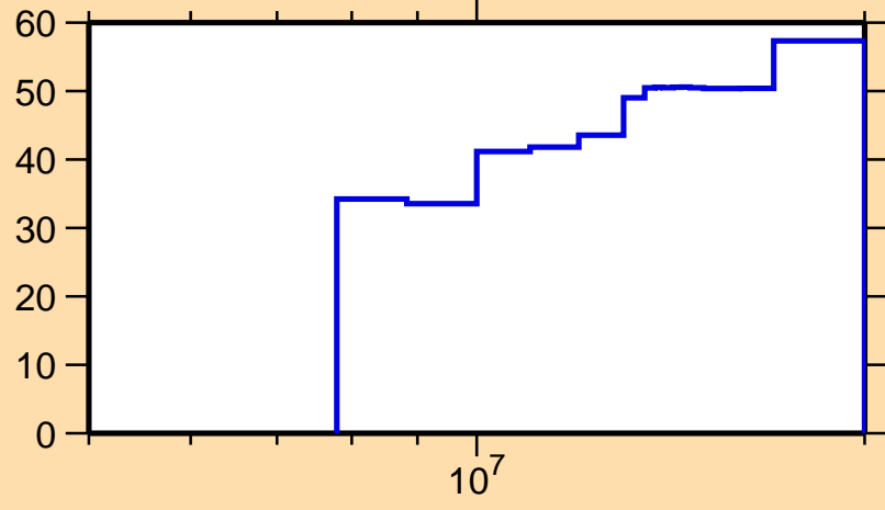
\Delta\sigma/\sigma vs. E for ^{134}\text{Te}(n,n\text{cont.})
