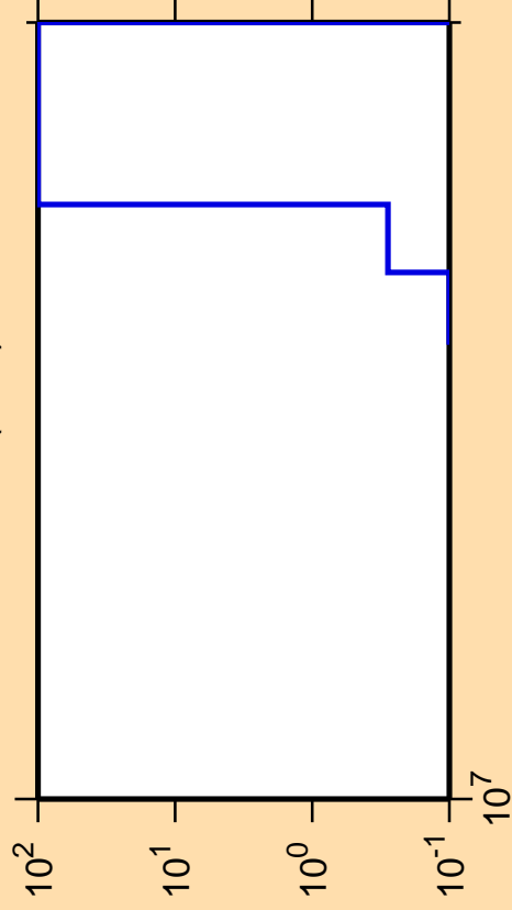
\Delta\sigma/\sigma vs. E for ^{134}\text{Te}(n,nt)
