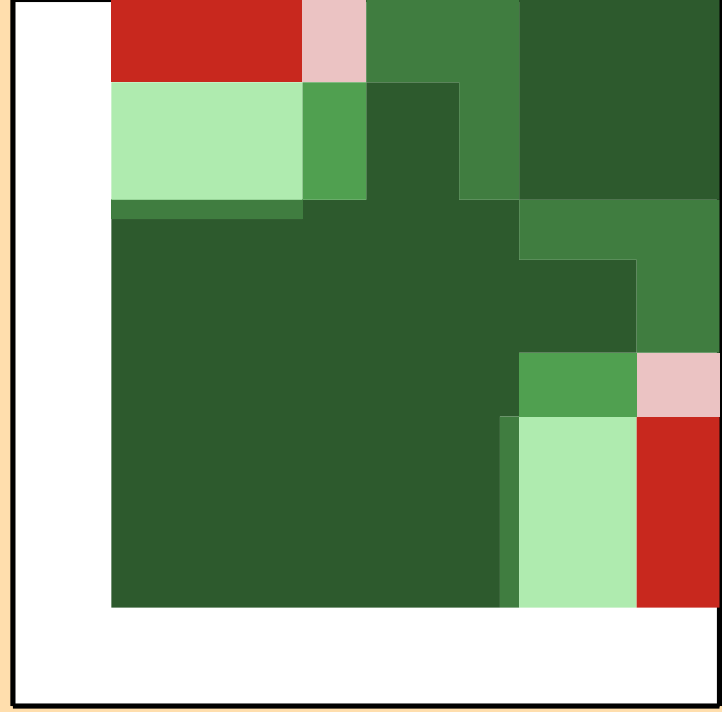
\sigma vs. E for ^{134}\text{Te}(n,n\text{cont.})
