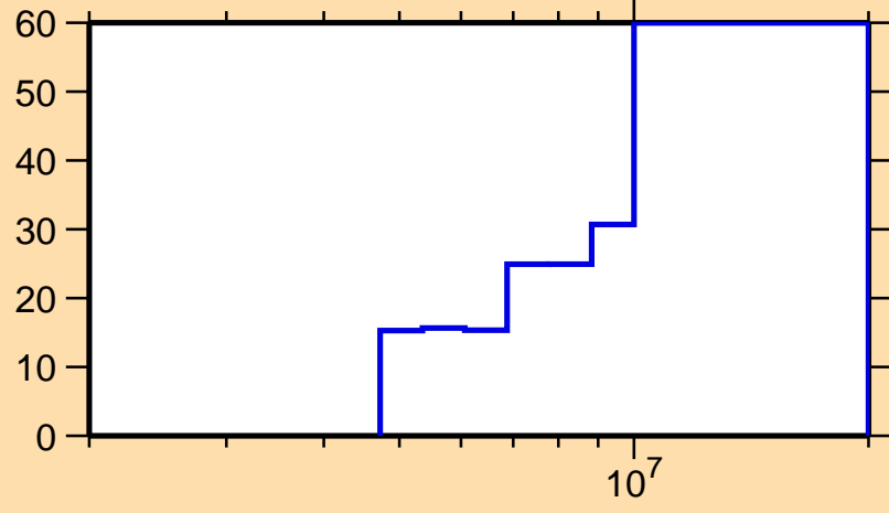
\Delta\sigma/\sigma vs. E for ^{134}\text{Te}(n,\text{inel.})
