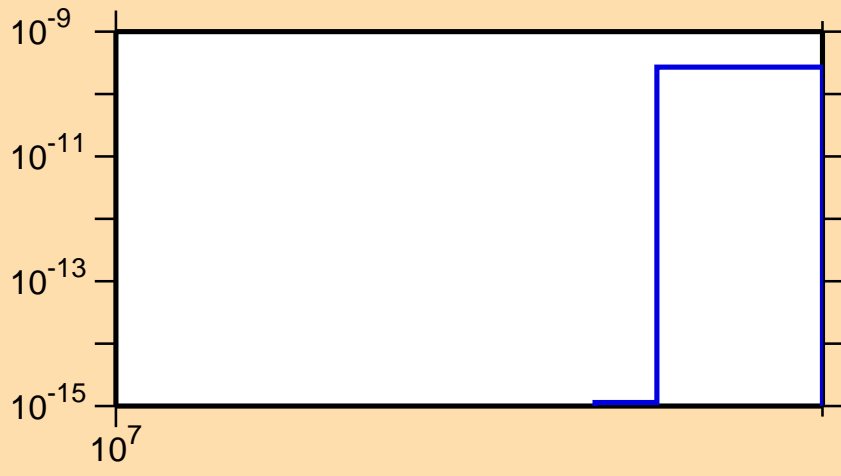
\sigma vs. E for ^{134}\text{Te}(n,\text{nd})
