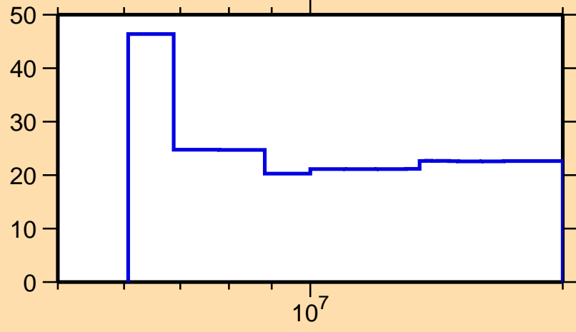
\Delta\sigma/\sigma vs. E for ^{134}\text{Te}(n,\text{el.})
