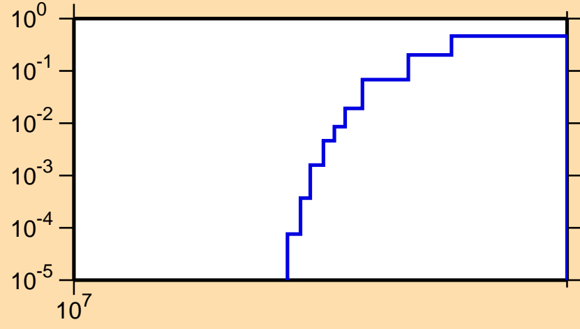
\sigma vs. E for ^{134}\text{Te}(n,3n)
