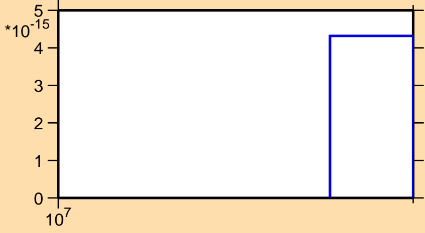
\sigma vs. E for ^{134}\text{Te}(n,2np)
