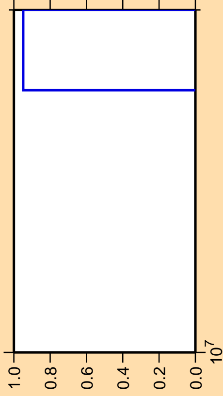
\Delta\sigma/\sigma vs. E for ^{134}\text{Te}(n,2n\alpha)
