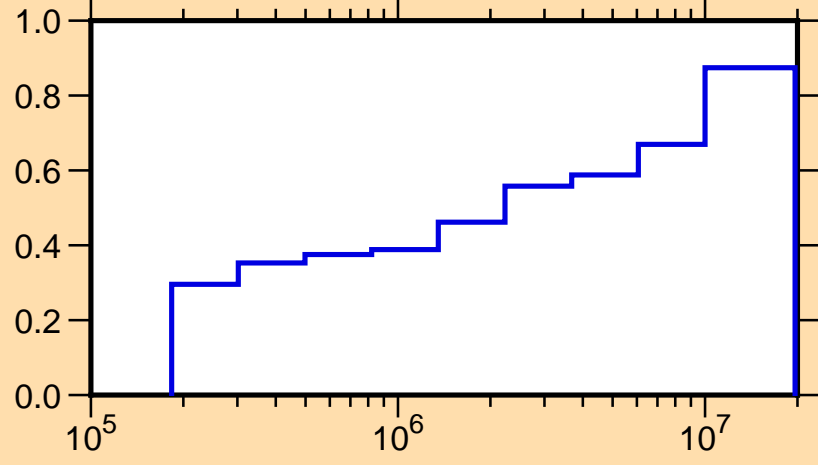
\mu vs. E for ^{134}\text{Te}(\text{mt251})
