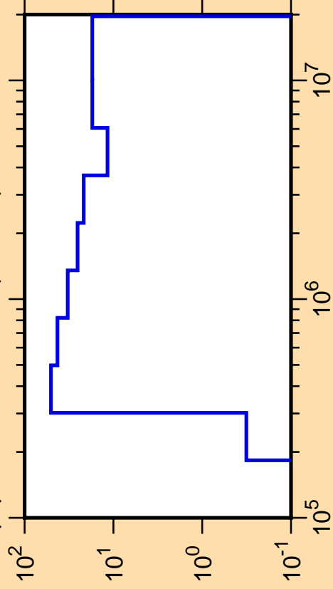
\Delta\mu/\mu vs. E for ^{134}\text{Te}(\text{mt251})
