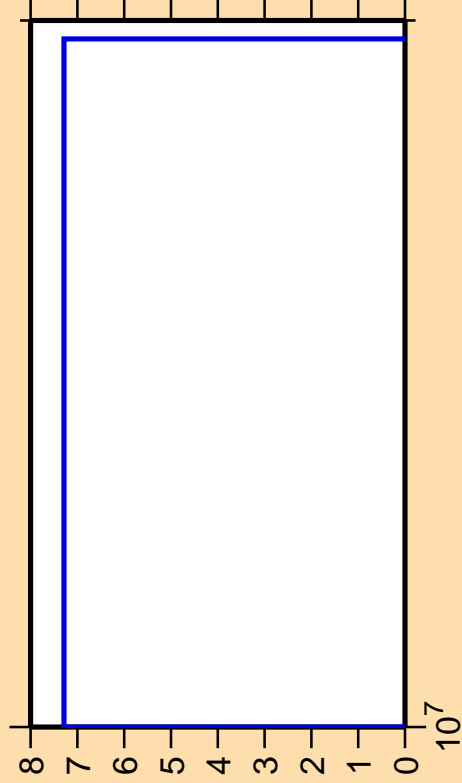
\Delta\sigma/\sigma vs. E for ^{134}\text{Te}(n,nd)
