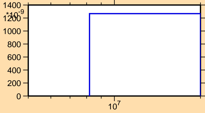
\sigma vs. E for ^{134}\text{Te}(n,t)
