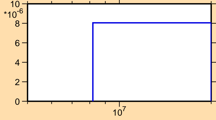
\sigma vs. E for ^{134}\text{Te}(n,np)
