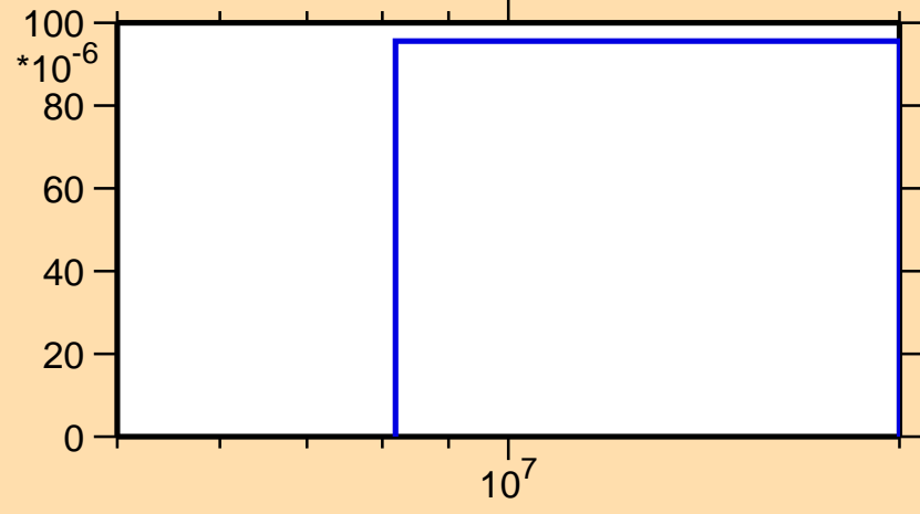
\sigma vs. E for ^{134}\text{Te}(n,p)
