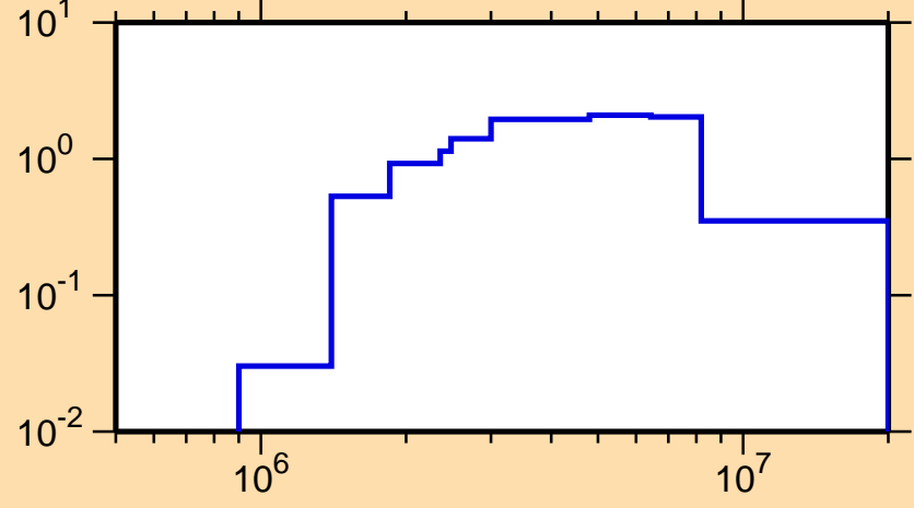
\sigma vs. E for ^{134}\text{Te}(n,\text{inel.})
