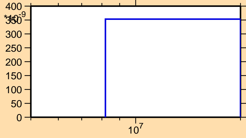
\sigma vs. E for ^{134}\text{Te}(n,\alpha)
