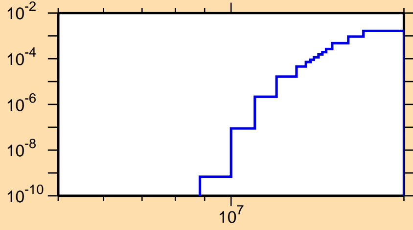
\sigma vs. E for ^{135}\text{Te}(n,p)
