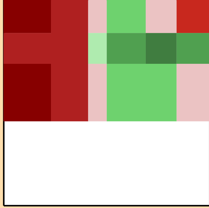
\Delta\sigma/\sigma vs. E for ^{135}\text{Te}(n,\gamma)
