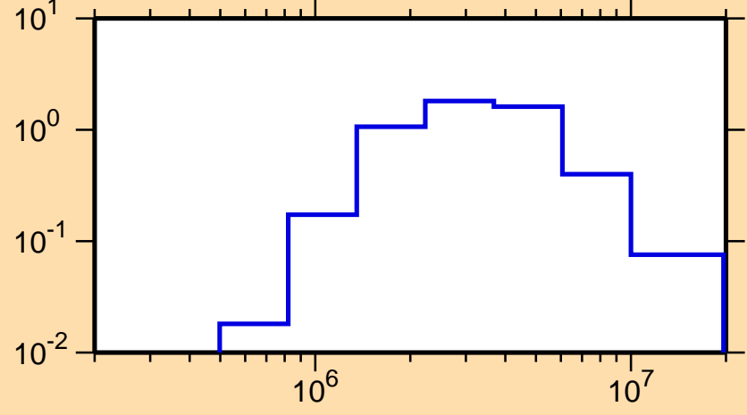
\sigma vs. E for ^{135}\text{Te}(n,\text{inel.})
