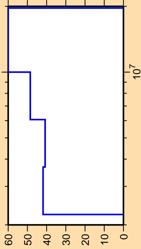
\Delta\sigma/\sigma vs. E for ^{135}\text{Te}(n,\text{ncont.})
