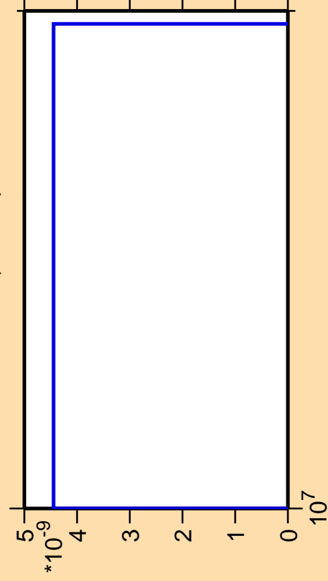
\Delta\sigma/\sigma vs. E for ^{135}\text{Te}(\text{mt } 11)
