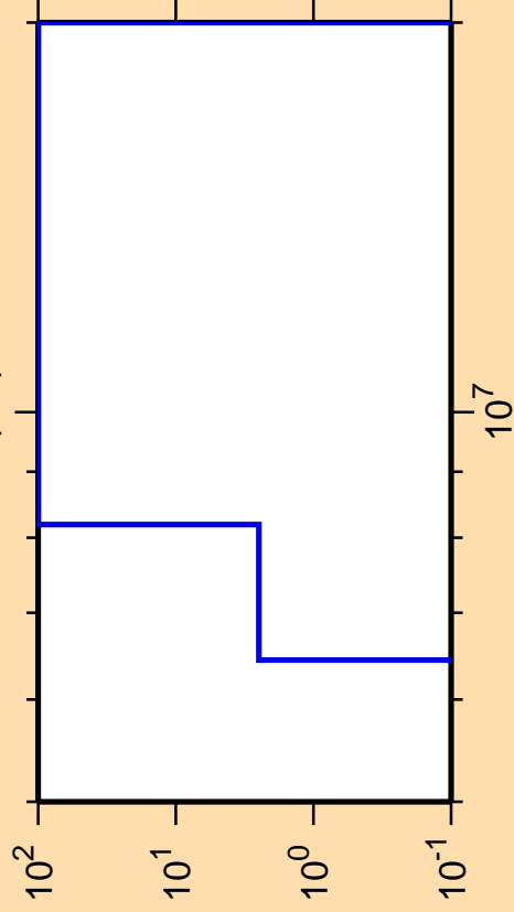
\Delta\sigma/\sigma vs. E for ^{135}\text{Te}(n,t)
