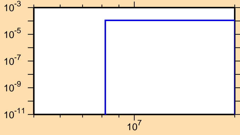
\sigma vs. E for ^{135}\text{Te}(n,t)
