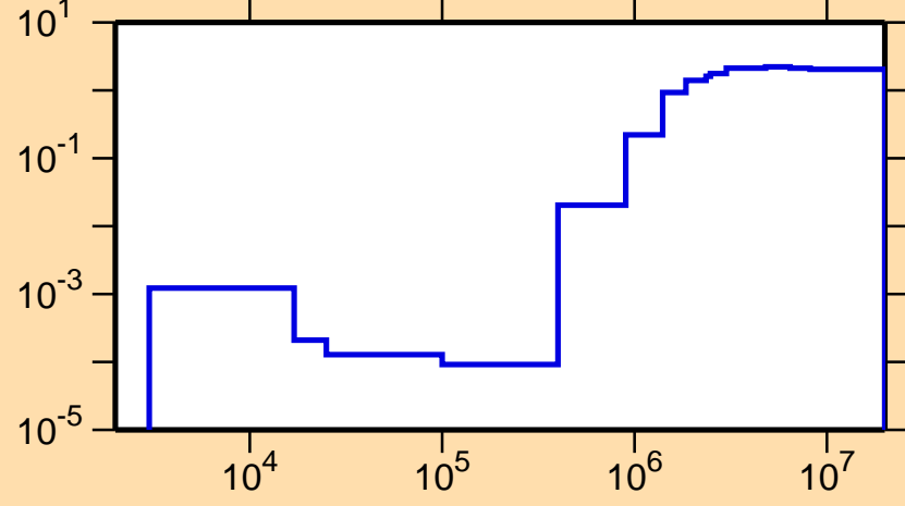
\sigma vs. E for ^{135}\text{Te}(n,\text{nonel.})
