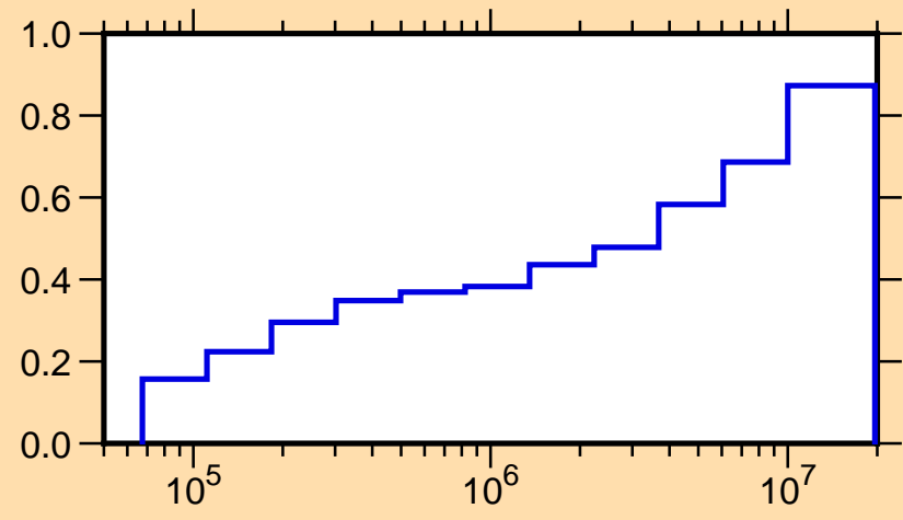
\mu vs. E for ^{137}\text{Te}(\text{mt251})
