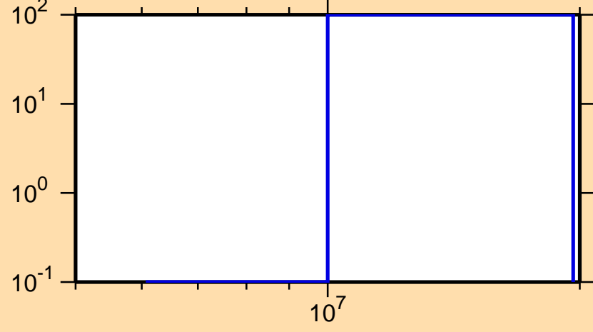
\Delta\sigma/\sigma vs. E for ^{137}\text{Te}(n,p)
