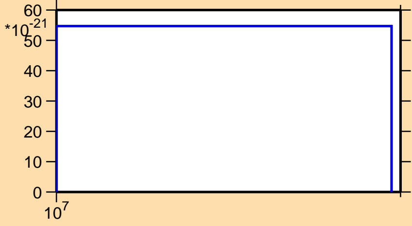
\sigma vs. E for ^{137}\text{Te}(\text{mt } 42)
