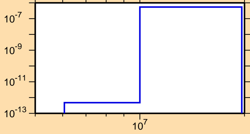
\sigma vs. E for ^{137}\text{Te}(n,2n\alpha)
