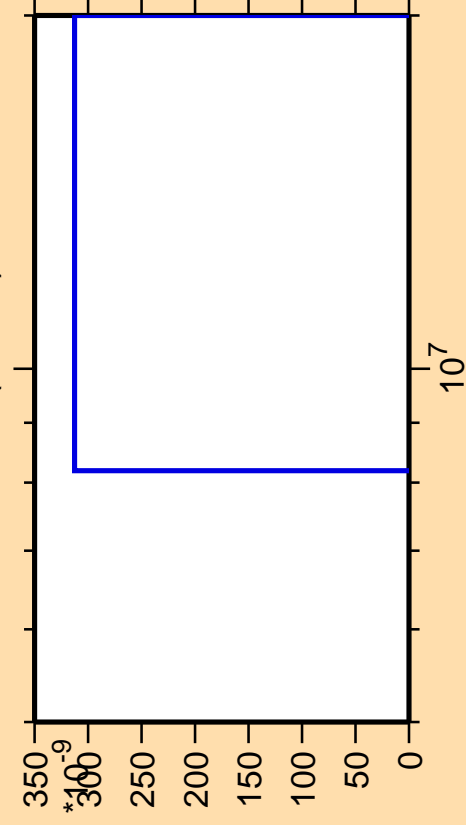
\Delta\sigma/\sigma vs. E for ^{137}\text{Te}(\text{mt } 42)
