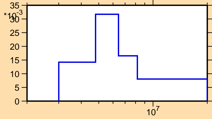
\sigma vs. E for ^{137}\text{Te}(n,n\text{cont.})
