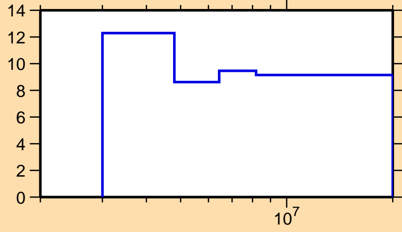
\Delta\sigma/\sigma vs. E for ^{137}\text{Te}(n,n\text{onel.})
