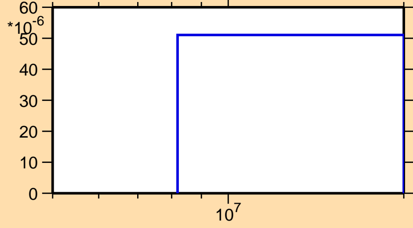
\sigma vs. E for ^{137}\text{Te}(n,p)
