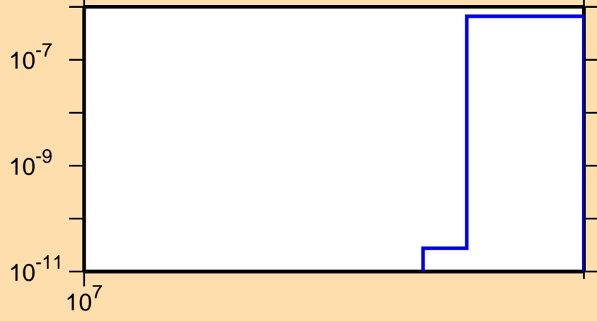
\sigma vs. E for ^{44}\text{Ti} (mt 45)
