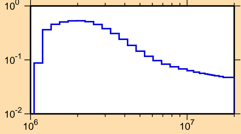
\sigma vs. E for ^{44}\text{Ti}(n,n_1)
