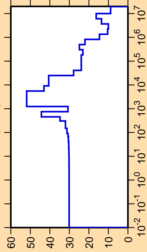
\Delta\sigma/\sigma vs. E for ^{44}\text{Ti}(n,\text{el.})
