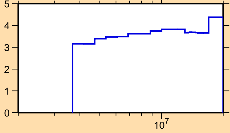
\Delta\sigma/\sigma vs. E for ^{46}\text{Ti}(n,\text{nonel.})
