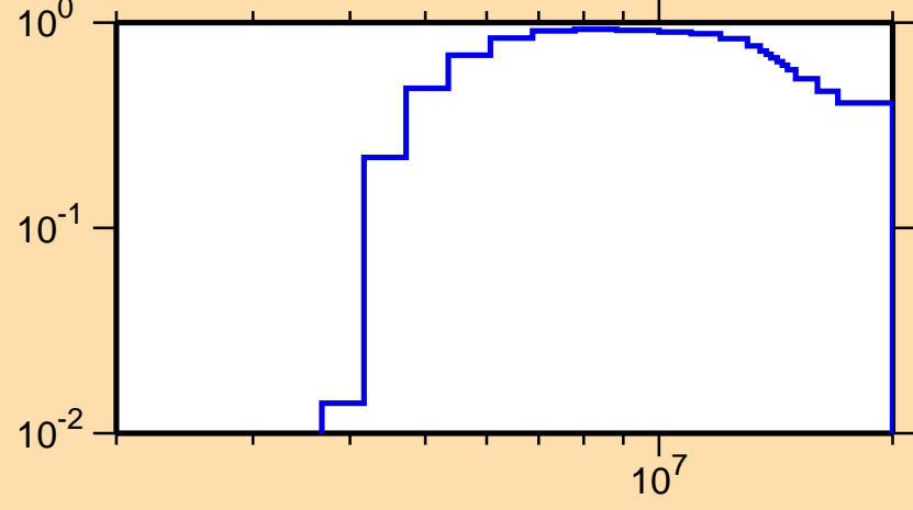
\sigma vs. E for ^{46}\text{Ti}(n,n\text{cont.})
