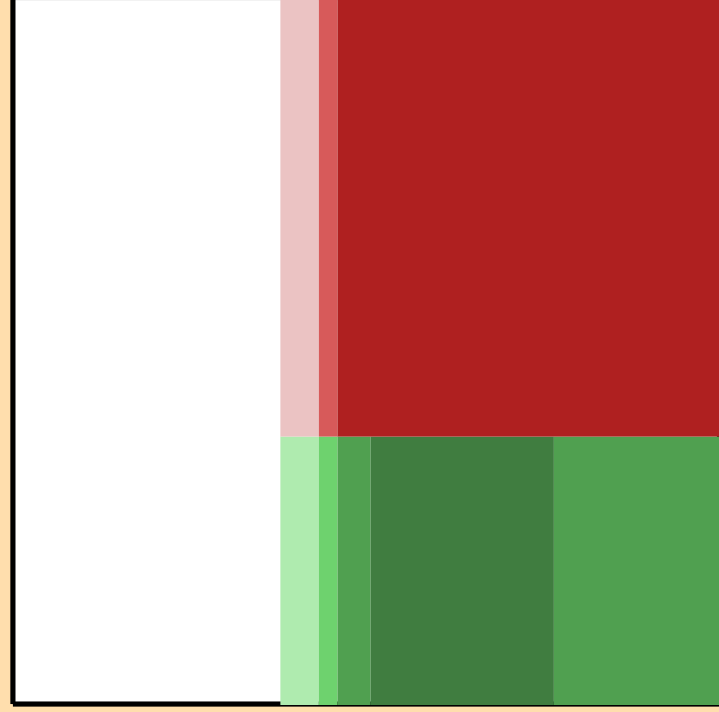
\Delta\sigma/\sigma vs. E for ^{46}\text{Ti}(n,2n)
