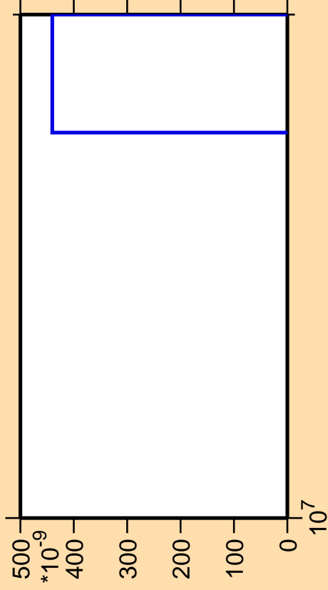
\Delta\sigma/\sigma vs. E for ^{46}\text{Ti}(n,nd)
