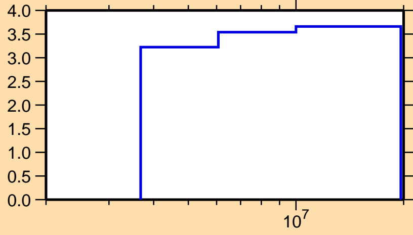
\Delta\sigma/\sigma vs. E for ^{46}\text{Ti}(n,n\text{nonel.})
