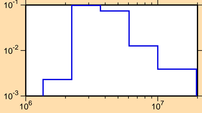
\sigma vs. E for ^{46}\text{Ti}(n,n_2)
