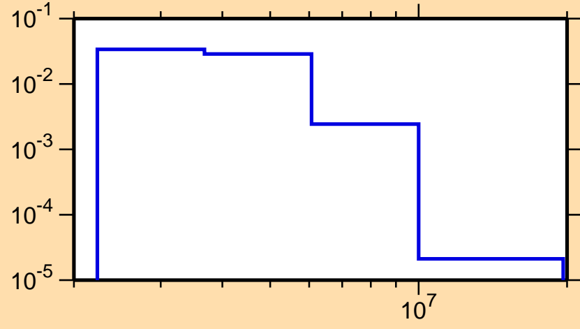
\sigma vs. E for ^{46}\text{Ti}(n,n_3)
