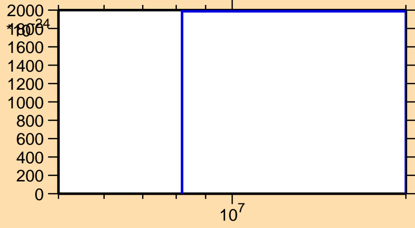
\sigma vs. E for ^{46}\text{Ti}(n,\text{nd})
