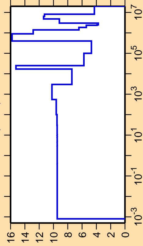
\Delta\sigma/\sigma vs. E for ^{46}\text{Ti}(n,\text{el.})
