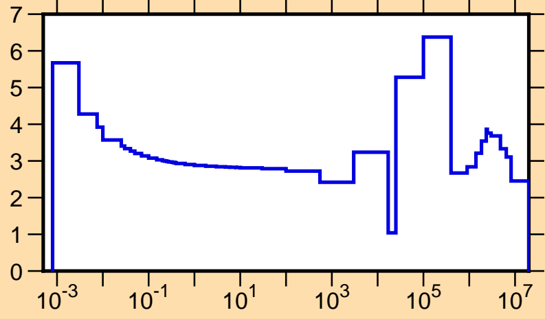
\sigma vs. E for ^{46}\text{Ti}(n,\text{tot.})
