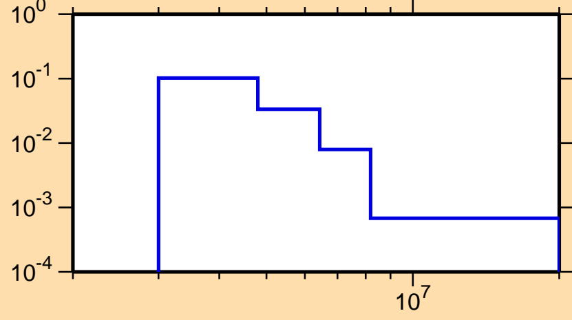
\sigma vs. E for ^{46}\text{Ti}(n,n_4)
