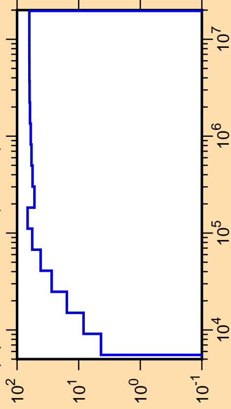
\Delta\mu/\mu vs. E for ^{47}\text{Ti}(\text{mt251})
