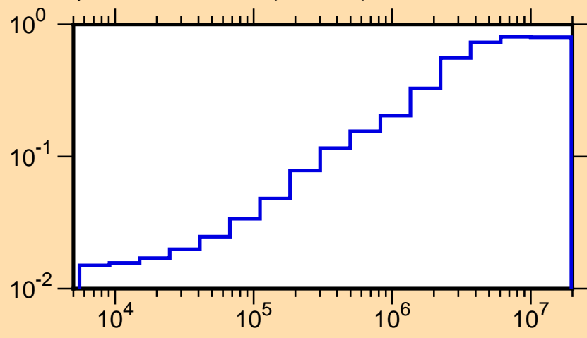
\mu vs. E for ^{47}\text{Ti}(\text{mt251})
