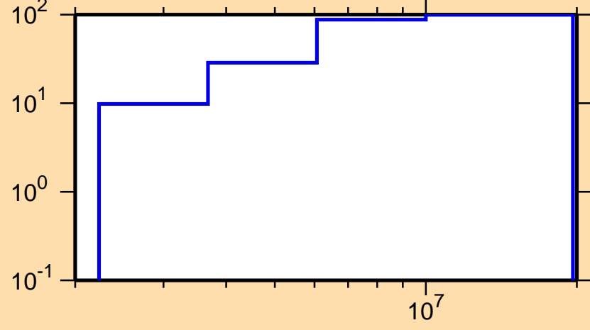
\Delta\sigma/\sigma vs. E for ^{47}\text{Ti}(n,n_1)
