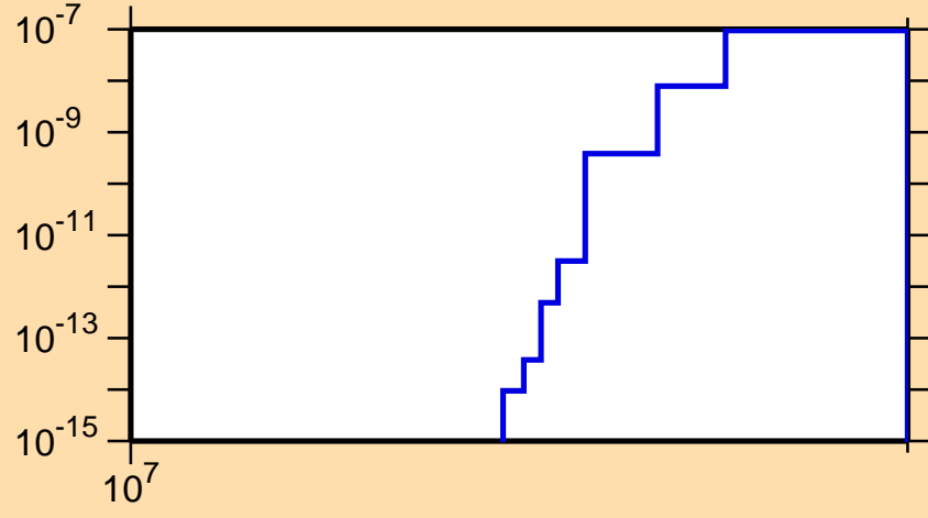
\sigma vs. E for ^{48}\text{Ti}(n,\text{He}3)
