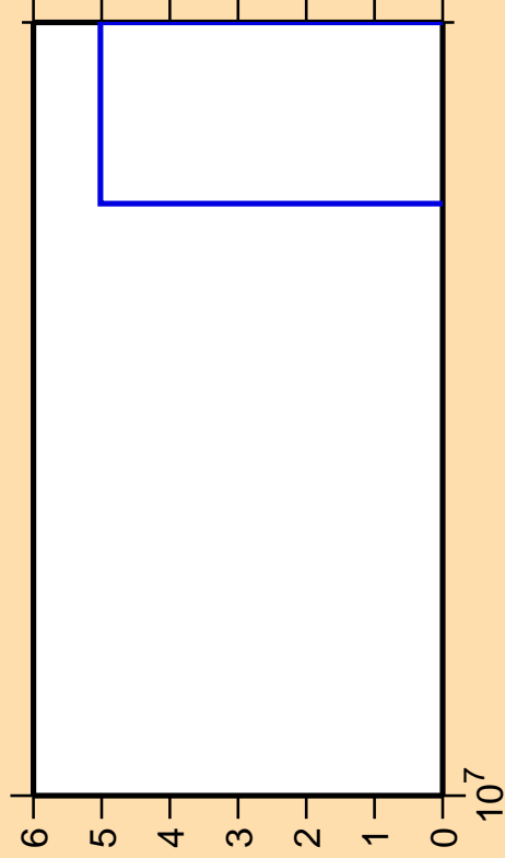
\Delta\sigma/\sigma vs. E for ^{48}\text{Ti}(n,\text{pd})
