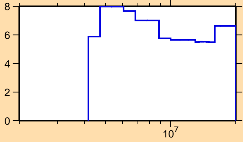
\Delta\sigma/\sigma vs. E for ^{48}\text{Ti}(n,n\text{onel.})
