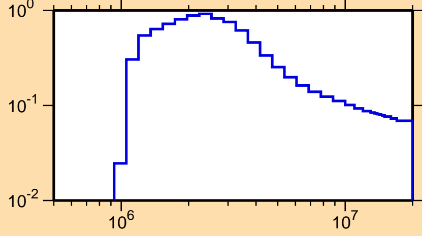
\sigma vs. E for ^{48}\text{Ti}(n,n_1)
