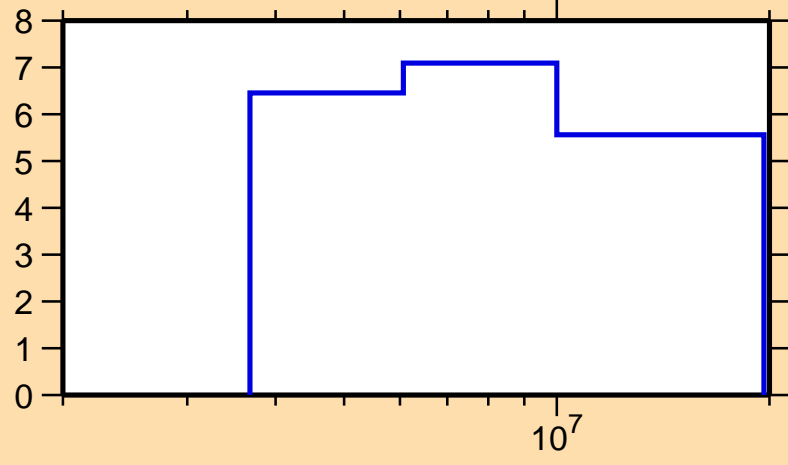
\Delta\sigma/\sigma vs. E for ^{48}\text{Ti}(n,n\text{nonel.})
