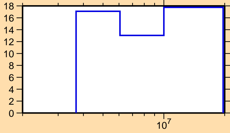
\Delta\sigma/\sigma vs. E for ^{48}\text{Ti}(n,ncont.)
