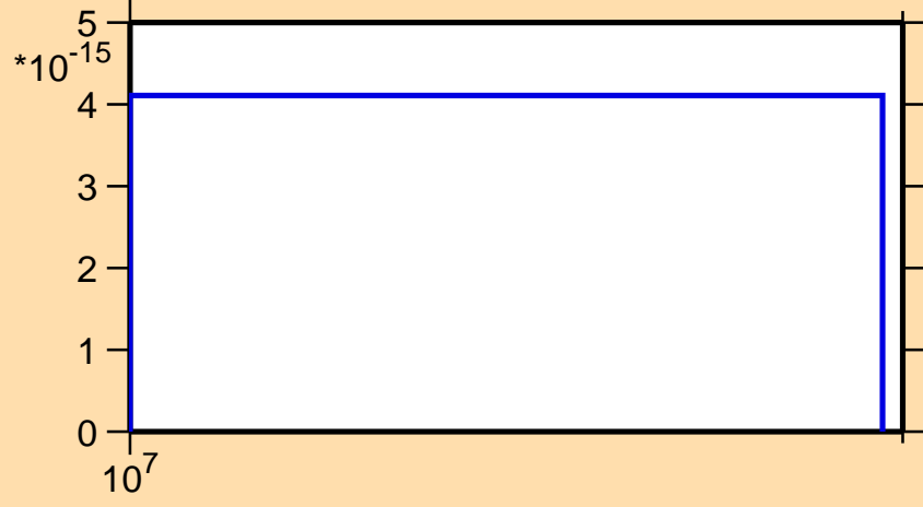
\sigma vs. E for ^{48}\text{Ti}(n,\text{pd})
