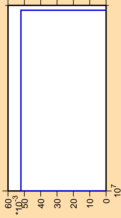
\Delta\sigma/\sigma vs. E for ^{48}\text{Ti}(n,\text{pd})
