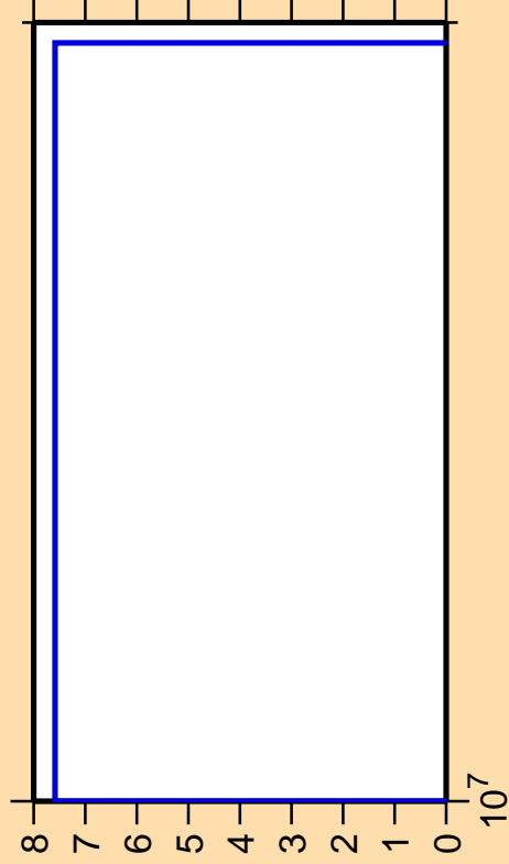
\Delta\sigma/\sigma vs. E for ^{48}\text{Ti}(n,p)
