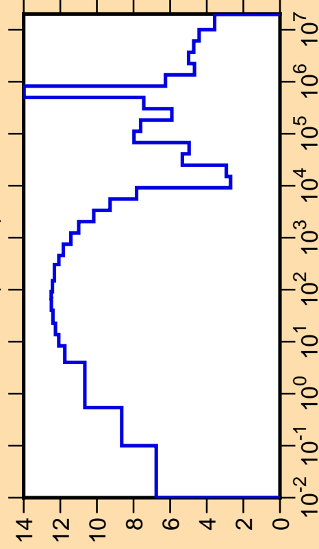
\Delta\sigma/\sigma vs. E for ^{48}\text{Ti}(n,\text{tot.})
