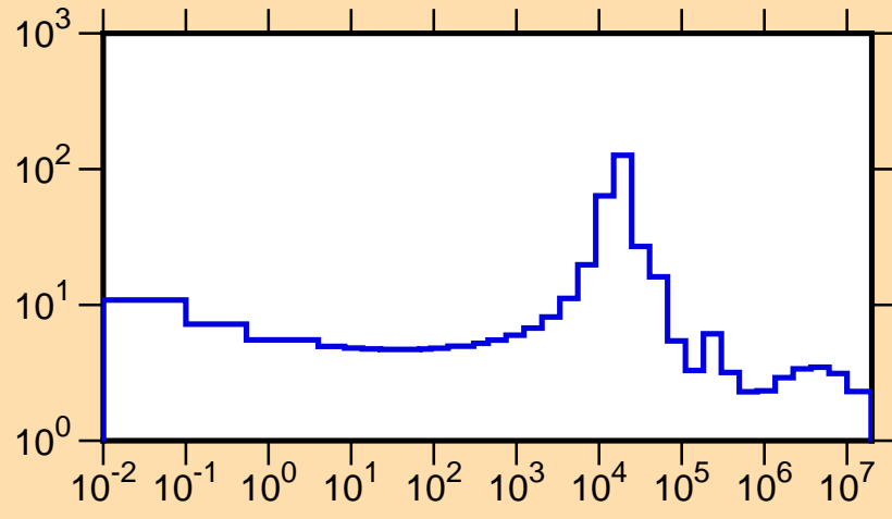
\sigma vs. E for ^{48}\text{Ti}(n,\text{tot.})
