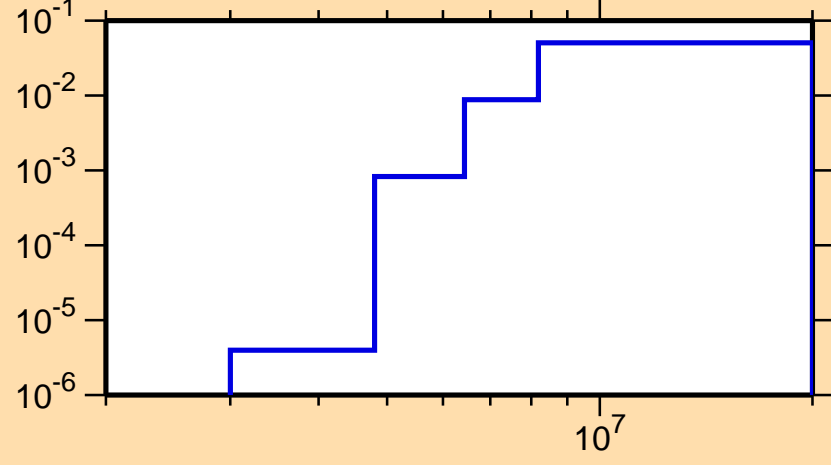
\sigma vs. E for ^{48}\text{Ti}(n,p)
