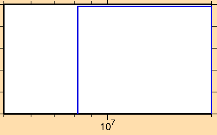
\sigma vs. E for ^{48}\text{Ti}(n,np)
