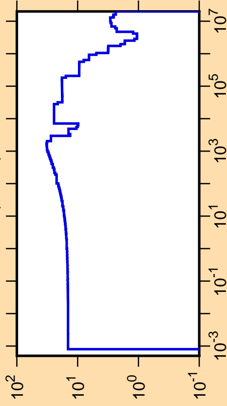
\Delta\sigma/\sigma vs. E for ^{48}\text{Ti}(n,\text{tot.})
