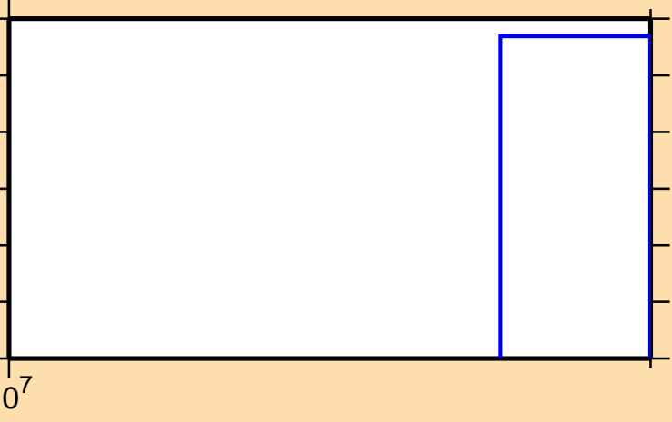
\sigma vs. E for ^{48}\text{Ti}(n,nt)
