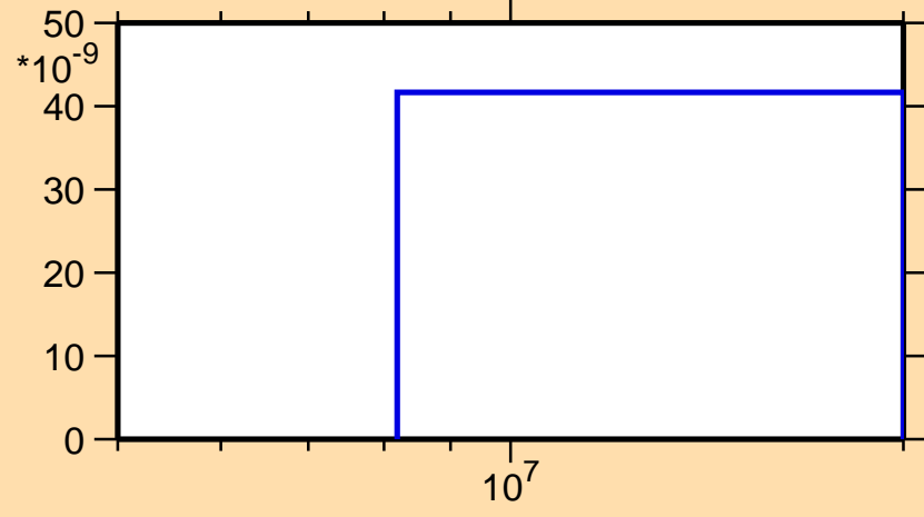
\sigma vs. E for ^{48}\text{Ti}(n,\text{nd})
