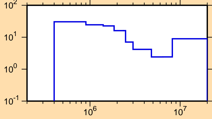
\Delta\sigma/\sigma vs. E for ^{48}\text{Ti}(n,n\text{cont.})
