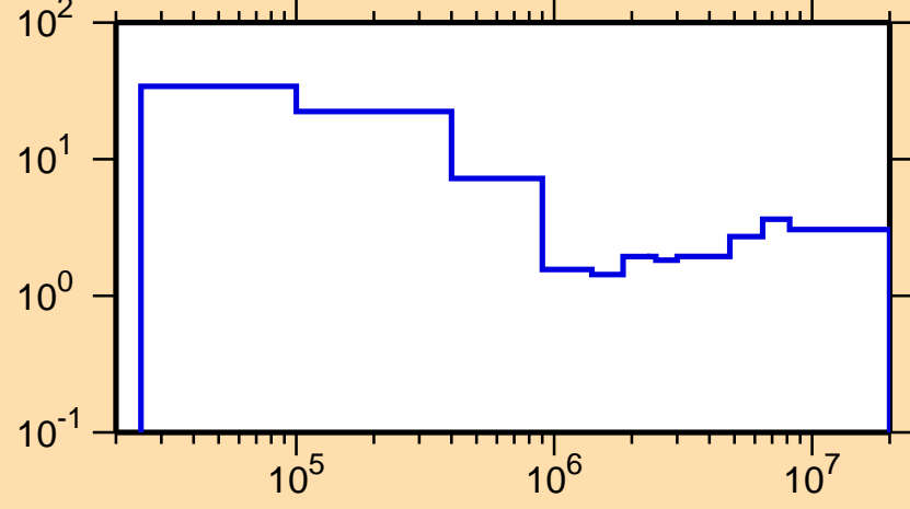
\Delta\sigma/\sigma vs. E for ^{48}\text{Ti}(n,el.)
