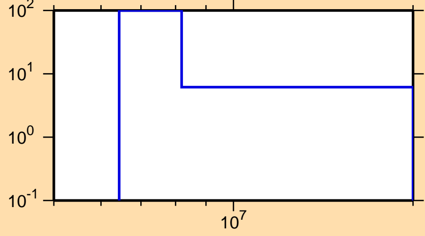
\Delta\sigma/\sigma vs. E for ^{48}\text{Ti}(n,2n)
