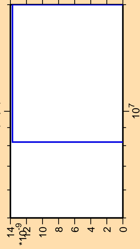
\Delta\sigma/\sigma vs. E for ^{48}\text{Ti}(n,\text{pt})
