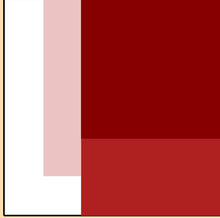
\Delta\sigma/\sigma vs. E for ^{48}\text{Ti}(n,2n)
