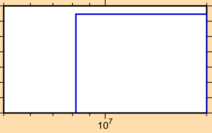
\sigma vs. E for ^{48}\text{Ti}(n,p\alpha)
