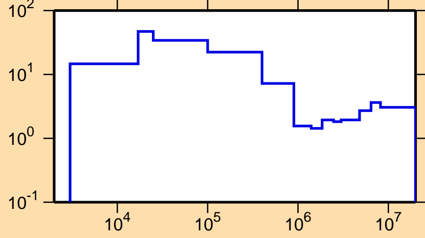
\Delta\sigma/\sigma vs. E for ^{48}\text{Ti}(n,\text{el.})
