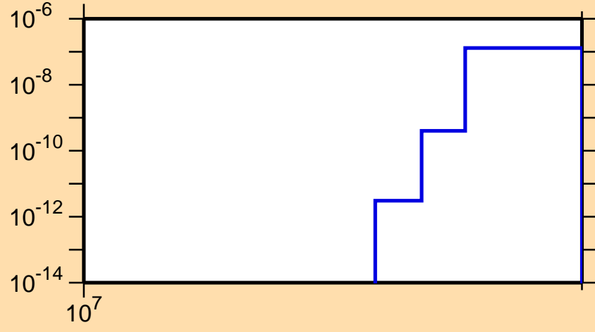
\sigma vs. E for ^{49}\text{Ti}(n,\text{He}3)
