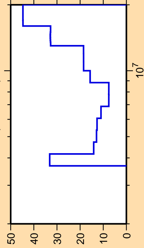
\Delta\sigma/\sigma vs. E for ^{49}\text{Ti}(n,ncont.)
