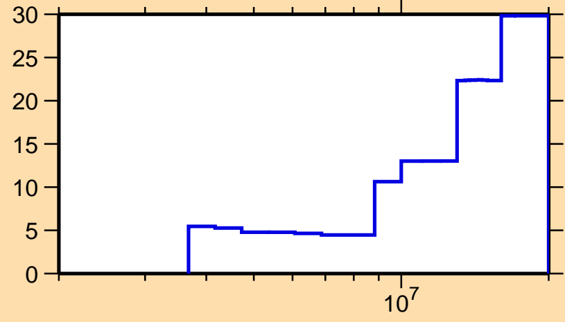
\Delta\sigma/\sigma vs. E for ^{49}\text{Ti}(n,inel.)
