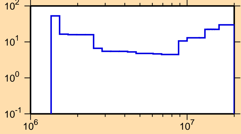
\Delta\sigma/\sigma vs. E for ^{49}\text{Ti}(n,\text{inel.})
