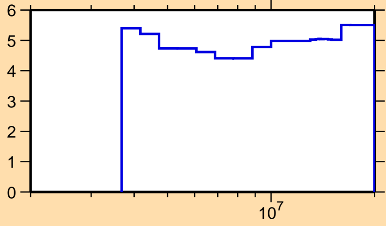
\Delta\sigma/\sigma vs. E for ^{49}\text{Ti}(n,n\text{nonel.})
