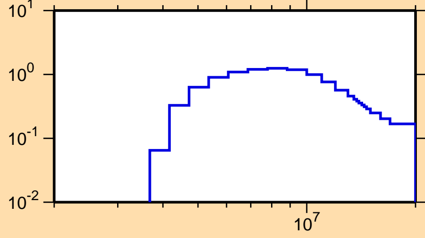
\sigma vs. E for ^{49}\text{Ti}(n,n\text{cont.})
