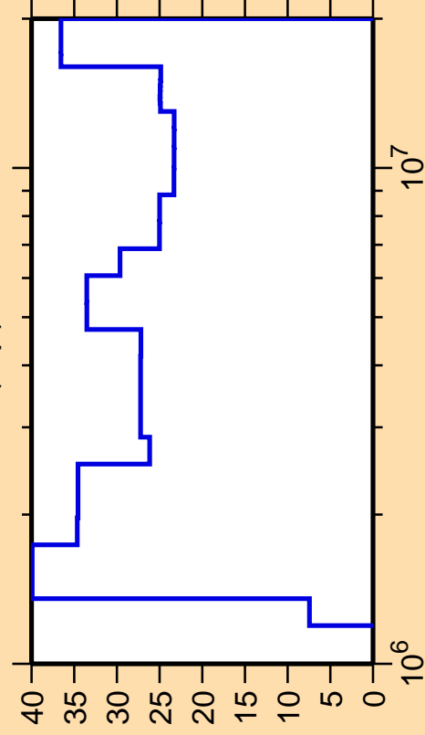
\Delta\sigma/\sigma vs. E for ^{49}\text{Ti}(n,p)
