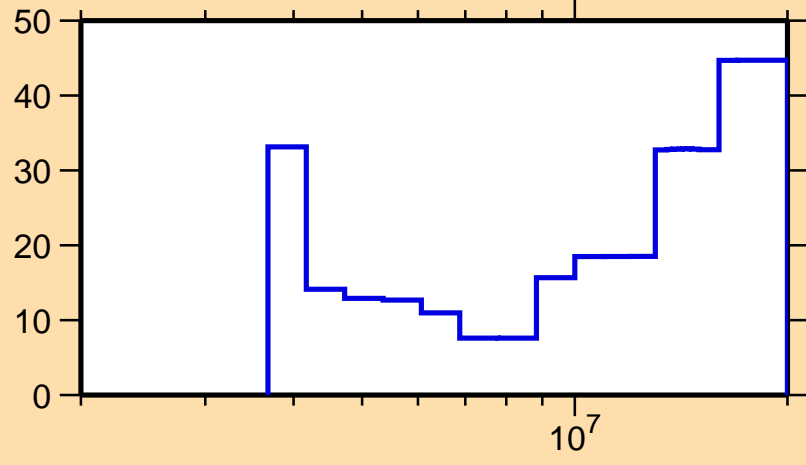
\Delta\sigma/\sigma vs. E for ^{49}\text{Ti}(n,n\text{cont.})
