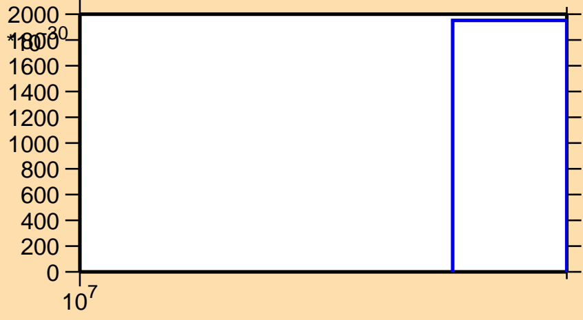
\sigma vs. E for ^{49}\text{Ti}(n,\text{pt})
