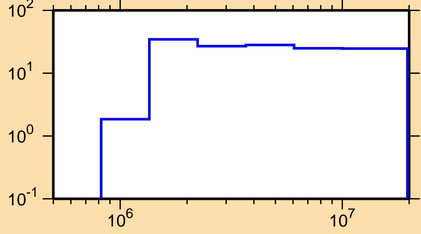
\Delta\sigma/\sigma vs. E for ^{49}\text{Ti}(n,p)
