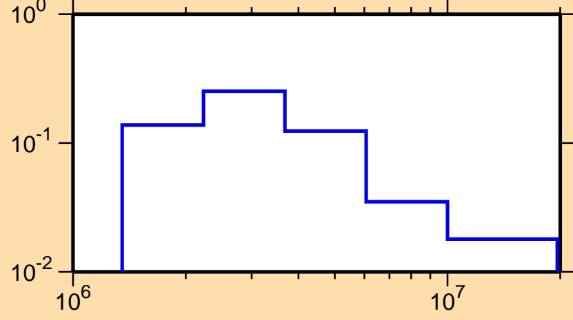
\sigma vs. E for ^{49}\text{Ti}(n,n_2)
