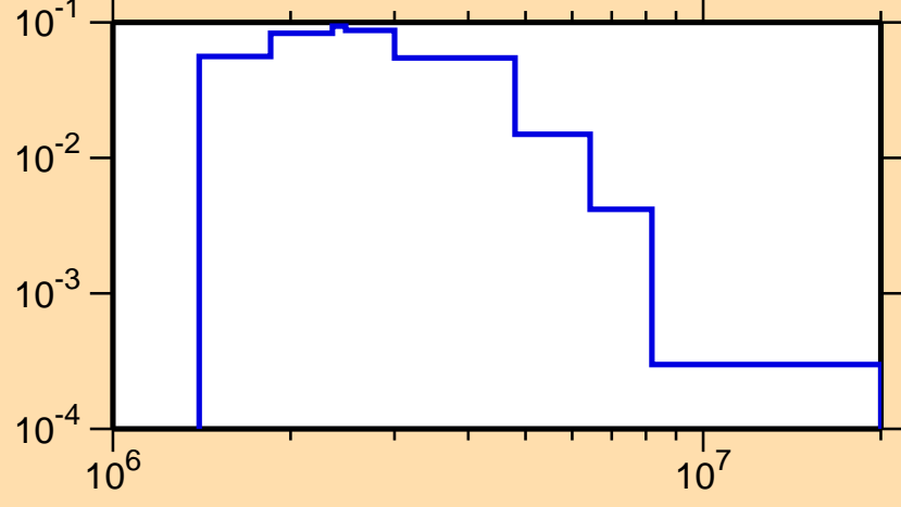
\sigma vs. E for ^{49}\text{Ti}(n,n_1)
