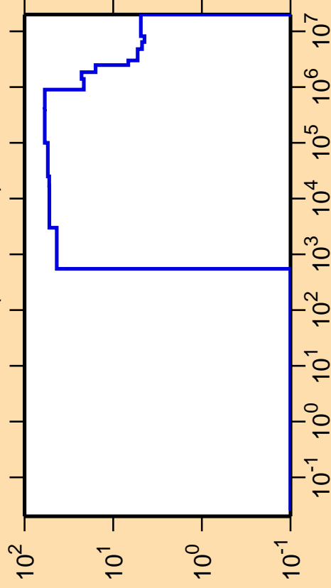
\Delta\sigma/\sigma vs. E for ^{49}\text{Ti}(n,\text{nonel.})
