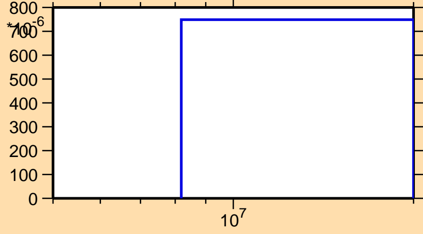
\sigma vs. E for ^{49}\text{Ti}(n,d)
