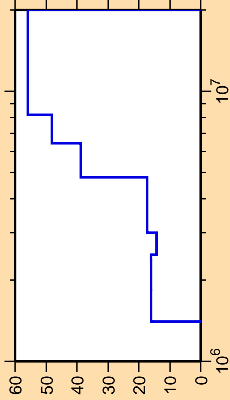
\Delta\sigma/\sigma vs. E for ^{49}\text{Ti}(n,n_1)
