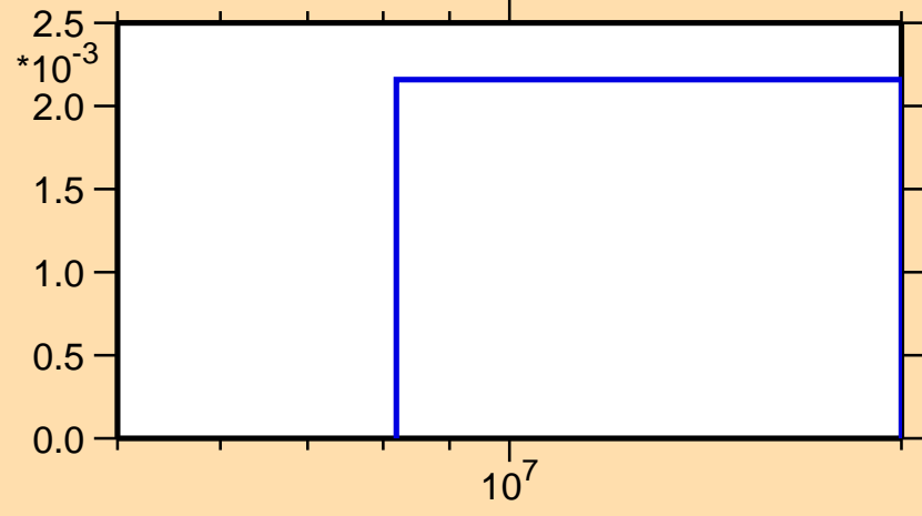
\sigma vs. E for ^{49}\text{Ti}(n,np)
