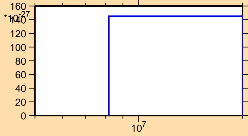
\sigma vs. E for ^{50}\text{Ti}(n,\text{pd})
