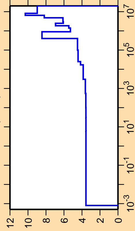
\Delta\sigma/\sigma vs. E for ^{50}\text{Ti}(n,\text{el.})
