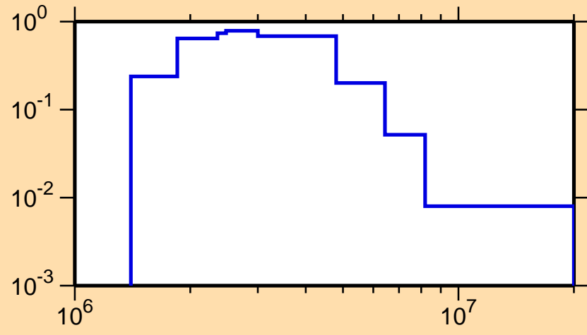
\sigma vs. E for ^{50}\text{Ti}(n,n_1)
