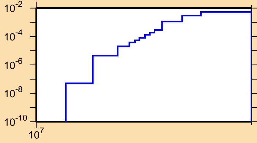
\sigma vs. E for ^{51}\text{Ti}(n,d)
