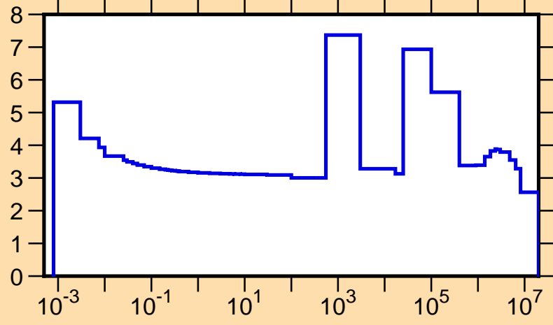
\sigma vs. E for ^{51}\text{Ti}(n,\text{tot.})
