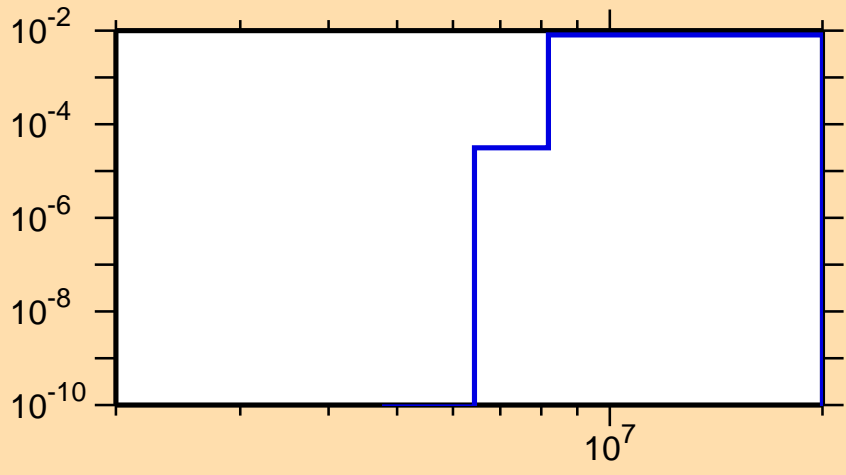
\sigma vs. E for ^{51}\text{Ti}(n,p)
