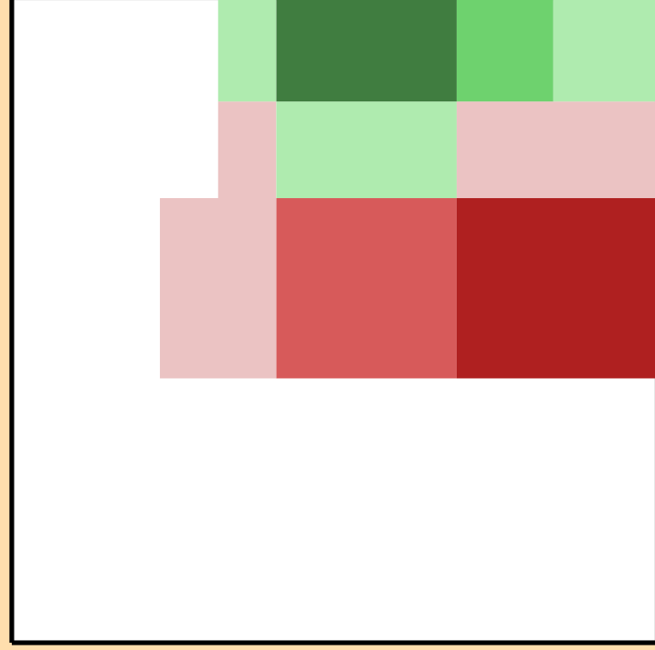
\Delta\sigma/\sigma vs. E for ^{52}\text{Ti}(n,ncont.)
