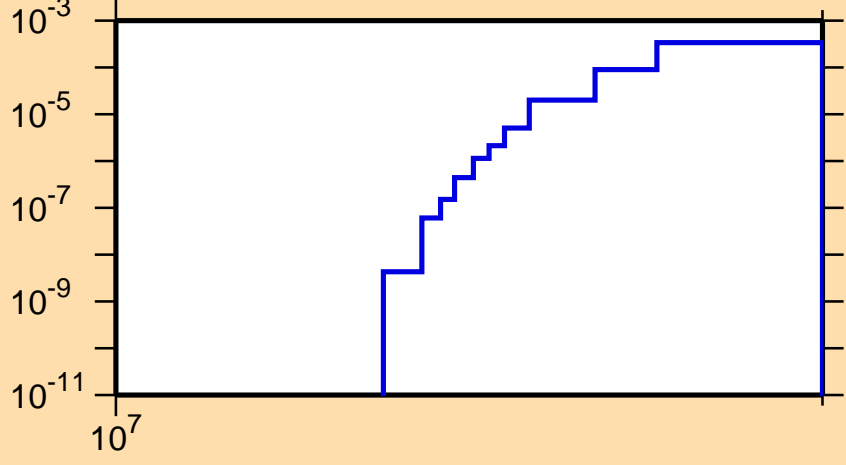
\sigma vs. E for ^{52}\text{Ti}(n,t)
