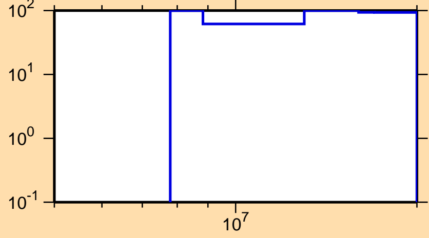
\Delta\sigma/\sigma vs. E for ^{52}\text{Ti}(n,p)
