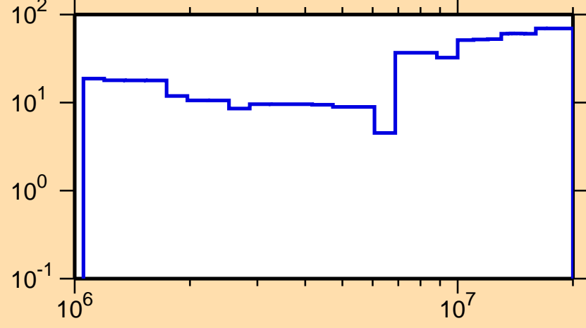
\Delta\sigma/\sigma vs. E for ^{52}\text{Ti}(n,\text{inel.})
