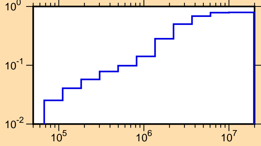
\mu vs. E for ^{52}\text{Ti}(\text{mt251})
